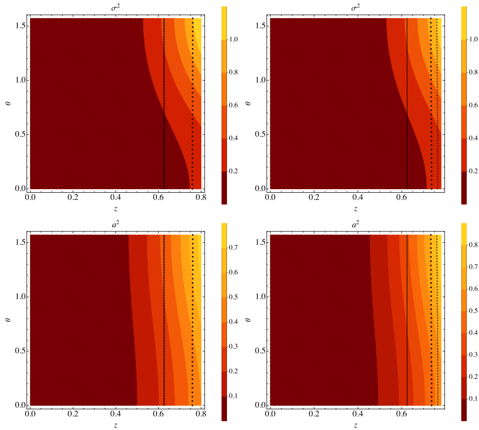
Figure 16. Figure showing the shear squared, \sigma_{\mu\nu}\sigma^{\mu\nu} , (top) and acceleration squared, a_\mu a^\mu (bottom) for the families IA (left) and IIB (right) for black holes with j = 0.8 in the limit \epsilon \rightarrow 0 . These are calculated using extrapolation to \epsilon = 0 from our small \epsilon solutions. The dashed, dotted and solid black lines show the spin 0, 1 and 2 horizons respectively of the last black hole solution with j = 0.8 that we have constructed, corresponding to \epsilon = 0.01 .
