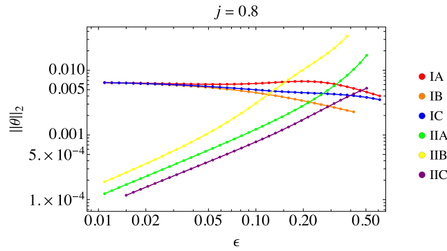
Figure 9. The L^2 -norm of the aether expansion over the coordinate range extending up to z_{\text{cut}} = 0.6 with j = 0.8 , vs \epsilon . For the region II families this norm vanishes linearly with \epsilon . For region I families the aether has a non-zero expansion as \epsilon \rightarrow 0 , which depends on the spin of the black hole but is independent of the coupling c_\omega .
