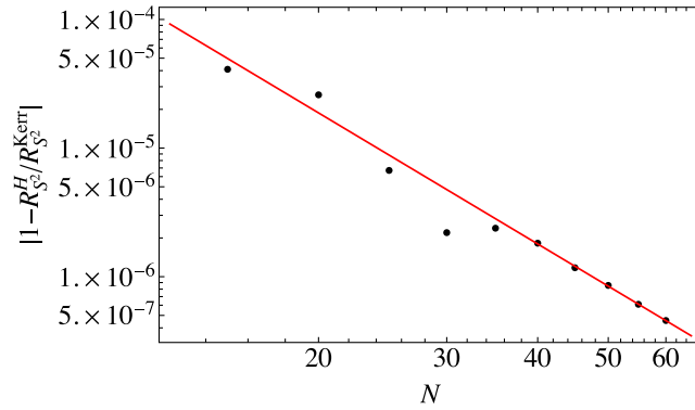
Figure 22. Convergence of the equatorial radius of the horizon S^2 for a Kerr black hole with j = 0.70 . The slope of the fit is -3.38 . Here N denotes the number of grid points along the z or \theta directions (we take them to be the same).
