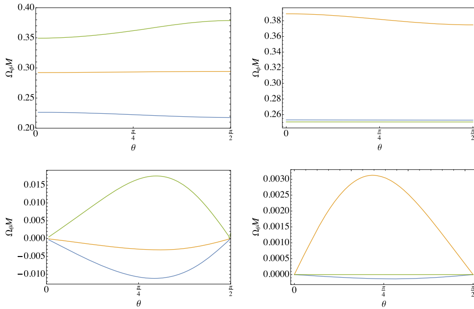
Figure 6. The angular velocities \Omega_\phi(\theta) and \Omega_\theta(\theta) , made dimensionless with the black hole mass M , for the wave mode horizons shown in figure 5. (Spin-0,1,2 horizon curves in left panels: lower, middle, upper; in top right panel: middle, upper lower; in bottom right panel: lower, upper, middle.) The non-vanishing \Omega_\theta(\theta) , and the explicit dependence of \Omega_\phi on \theta , show that these are not Killing horizons. The corresponding values for Kerr with the same mass and angular momentum are \Omega_H M = \{0.235, 0.250\} for the black holes on the {left, right}, respectively.
