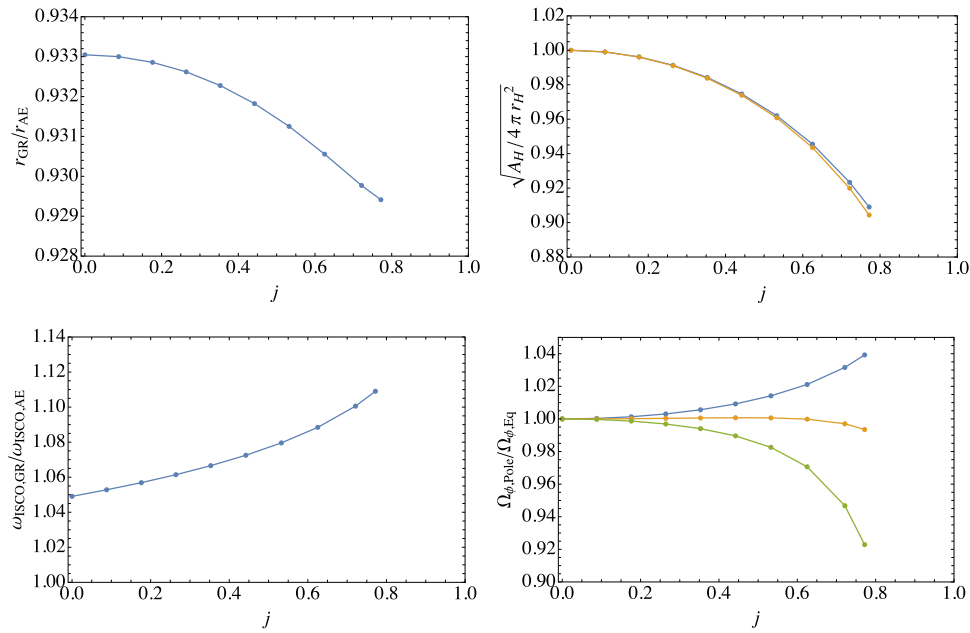
Figure 3. Comparison of properties of rotating Einstein-aether black holes with Kerr for the same spin and mass, for coupling parameters c_\omega = c_\sigma = c_a = 0.5 and c_\theta determined by s_0^2 = 1 (the same couplings as a case previously considered for static black holes in [15]). The top left plot shows the ratio of the equatorial horizon radius for Kerr to that of the aether black holes, vs spin j = J/M^2 . The top right plot shows \sqrt{A_H/4\pi r_H^2} with aether black holes in blue (upper) and Kerr in orange (lower). The lower left plot shows the ratio of the ISCO frequency for Kerr to the aether solutions. The lower right plot shows the ratios of the angular velocity \Omega_\phi at the pole to that at the equator for the spin-0 (blue, upper), 1 (orange, middle) and 2 (green, lower) wave mode horizons. These deviate from one since, unlike for the Kerr metric horizon, these are not Killing horizons.
