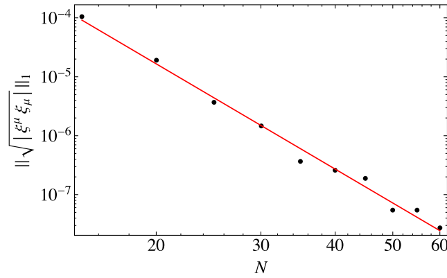
Figure 21. L_1 norm of \sqrt{|\xi^\mu \xi_\mu|} for a Kerr black hole with j = 0.70 and z_{\max} = 0.65 . The slope of the fit is -5.93 , indicating near sixth order convergence, as one would expect. Here N denotes the number of grid points along the z and \theta directions.
