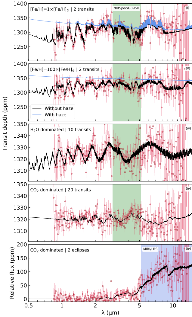
Fig. 15. Synthetic Webb atmospheric spectra of Gl 486b. Top to bottom : Transmission spectra under optimistic (i), feasible (ii), realistic and interior-compatible (iii), and realistic (iv) scenarios, and emission spectrum for the realistic (iv) scenario. Red circles with estimated uncertainties are shown for different numbers of transits and eclipses as stated in the panels, with Webb NIRISS/SOSS, NIRSpec/G395H, and MIRI/LRS configurations. Black and blue lines represent clear (i.e. no haze opacity contribution) and hazy atmospheres, respectively. There is no hazy atmosphere in the realistic scenarios. NIRSpec/G395H and MIRI/LRS (Table 11) wavelength coverages are highlighted by green and blue shades, respectively.
