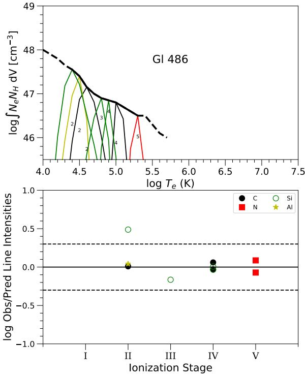
Fig. 8. Stellar coronal emission of GI 486 from ultraviolet spectroscopy. Top: emission measure distribution from Hubble /STIS data. Thin, coloured lines represent the relative contribution function for each ion (the emissivity function multiplied by the emission measure distribution at each point). Numbers within the graph indicate the ionisation stages of the species. Bottom: observed-to-predicted line flux ratios for the ion stages in the upper figure. The dashed lines denote a factor of two.
