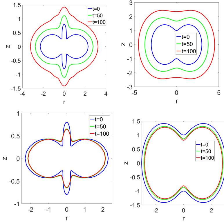
FIGURE 3. Axially symmetric 3-D tumors with W = w_0 and \lambda_T = 4 \times 10^{-3} . The top row with \eta = 1000 , \varepsilon = 0 , the bottom row with \eta = 10000 , \varepsilon = 0.9 . Tumor volumes increase in the top row, and decrease in the bottom row.
