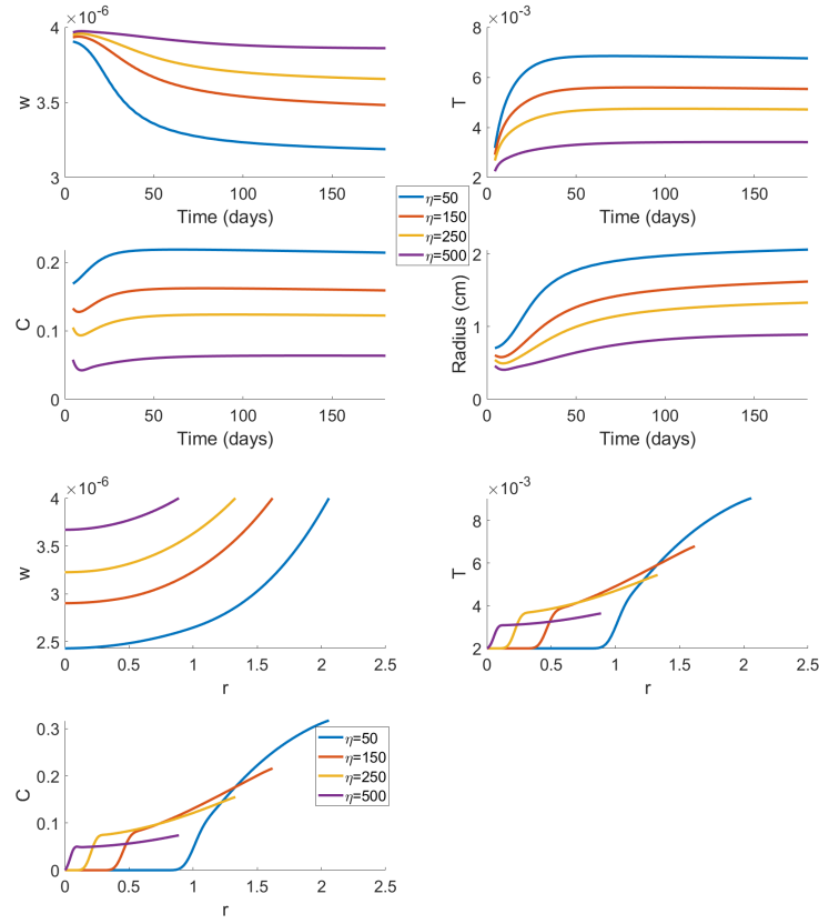
FIGURE 2. Treatment with VEGF inhibitor, immune checkpoint blockade, and cancer vaccine. W = w_0 on the free boundary, with \lambda_T = 4 \times 10^{-3} and \varepsilon = 2 . The first four figures describe the dynamic of the average density of w , T , C (in units of g/cm^3 ) within the tumor, and the radius growth during 180 days. The last three figures describe the densities of w , T , C along the radius of the tumor at day t = 180 .
