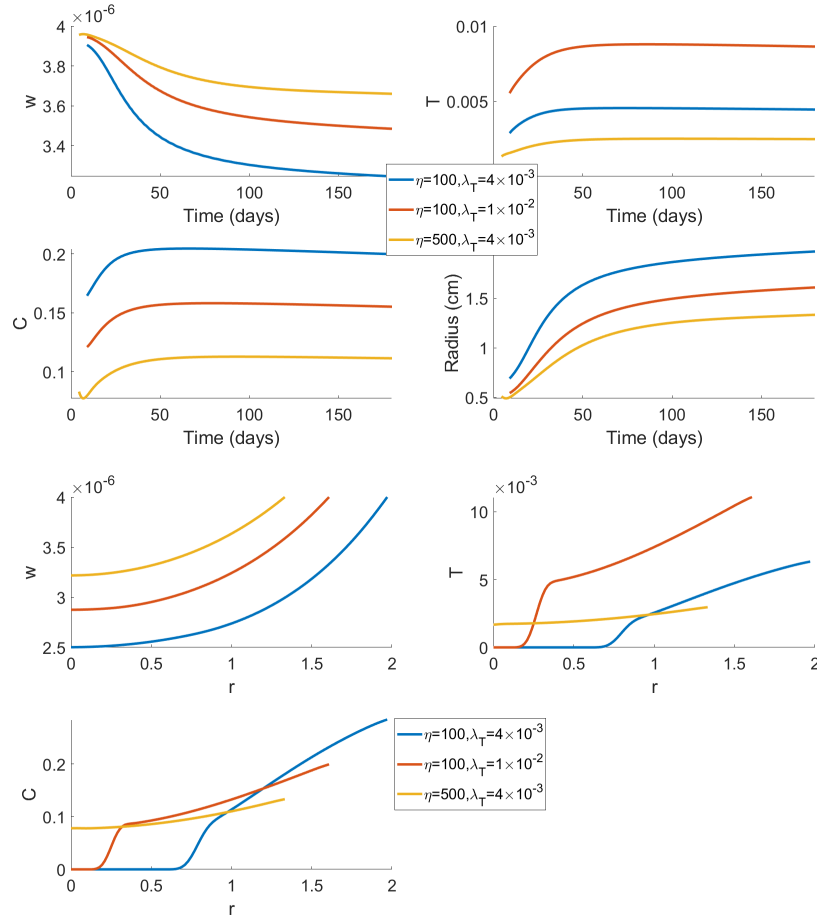
FIGURE 1. Treatment with VEGF inhibitor. W = w_0 on the free boundary, with \varepsilon = 0 and different \lambda_T and \eta . The first four figures describe the dynamic of the average density of w , T , C (in units of g/cm^3 ) within the tumor, and the radius growth during 180 days. The last three figures describe the densities of w , T , C along the radius of the tumor at day t = 180 .
