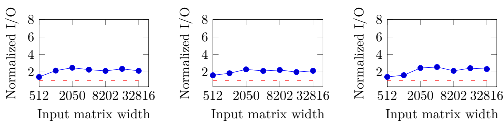
(a) 3 concurrent instances of the same size. (b) 3 concurrent instances of different sizes. (c) 3 concurrent instances each of MM-SCAN and MM-INPLACE.
