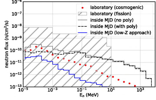
FIG. 12. (Color online) Neutron flux at the 4850ft level for various shielding scenarios. The red dots and the grey area curve show the neutron flux entering the experimental cavity from cosmogenics and due to fission in the rock [59]. The increase in flux after the innermost shielding layer of the DEMONSTRATOR (black dashed) is due to the production of additional neutrons by muons in lead. Different shielding approaches, e.g. no poly-shield (grey), or low-Z approach with liquid argon (blue) can affect the flux.
