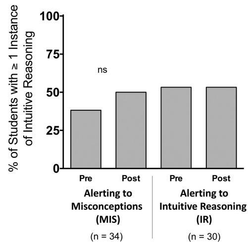
FIG 3. Time 2. Percentage of students producing intuitive language in response to the open-ended prompt “How would you explain antibiotic resistance to a fellow student in this class?” No statistically significant differences were observed in either intervention group.
