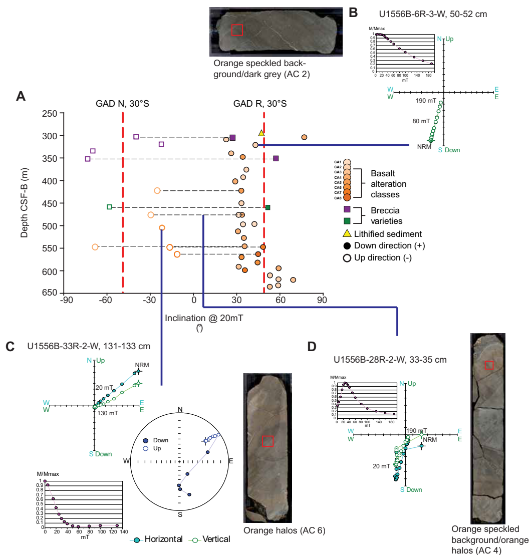
Figure F19. Stepwise demagnetization orthogonal vector plots, decay AF plot, and sampling location of cores for representative samples of different alteration classes along with both (A) ChRM and overprint inclinations of Hole U1556B discrete samples (B: no overprint, C: completely overprinted, D: partially overprinted).
