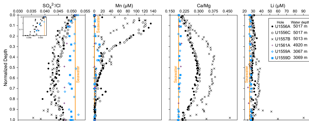
Figure F16. IW chemistry along SAT. Orange = standard seawater values ( \text{SO}_4^{2-}/\text{Cl} = 28 \text{ mM}/546 \text{ mM} , \text{Mn} = 0.36 \text{ μM} , \text{Ca}/\text{Mg} = 10.27 \text{ mM}/52.7 \text{ mM} , \text{Li} = 25.9 \text{ μM} ). Sediment depths were normalized to maximum sediment thickness of each hole to compare variations in IW chemical profiles (0 = near mudline, 1 = near basement). Inset on \text{SO}_4^{2-}/\text{Cl} plot shows depth dependent decrease in ratios in all holes between 0 and 0.15 normalized depth. Standard seawater values were taken from Monterey Bay Aquarium Research Institute (MBARI) Periodic Table of Elements in the Ocean ( https://www.mbari.org/science/upper-ocean-systems/chemical-sensor-group/periodic-table-of-elements-in-the-ocean ).
