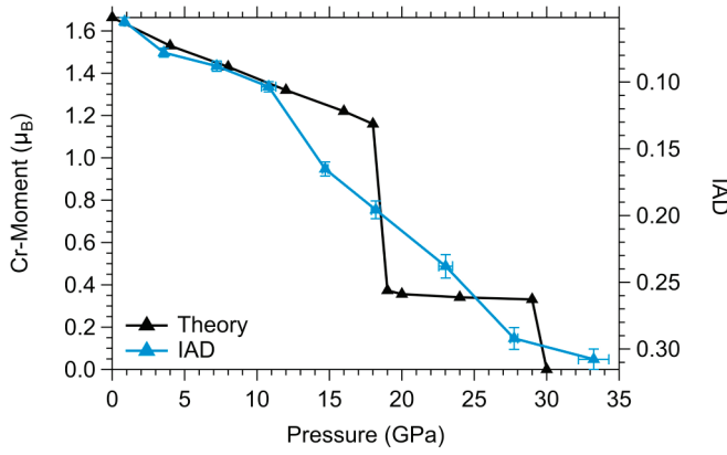
FIG. 7. Comparison of experimental IAD values with the predicted pressure dependence of the Cr moment [6]. The low-pressure region agrees well, but our measurements show a steady decline in the Cr moment rather than two steplike features.
