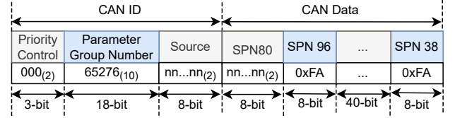
Figure 7: Attack Packet for Case Study 1
