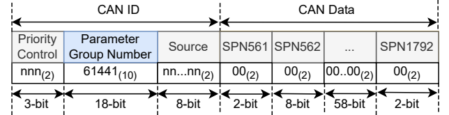
Figure 9: Attack Packet for Case Study 2
