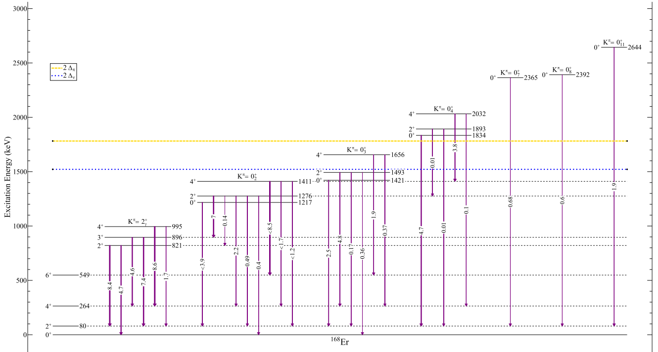
FIG. 4. Partial level scheme for the 0^+ bands identified and discussed in this work. The solid arrows represent E2 transitions. The upper limits of the transition probabilities are given in Table I. The band labels are according to the (p, \pi) experiment labels [6]. The dotted horizontal lines are the two-neutron and two-proton pairing gaps for ^{168}\text{Er} calculated using the formulas in Ref. [40] and masses from Ref. [41].
