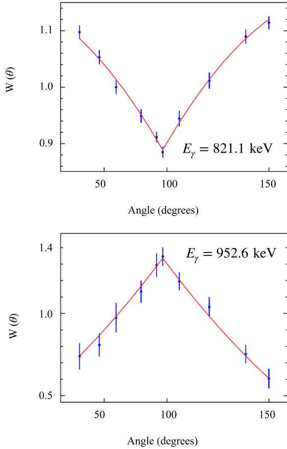
FIG. 2. Angular distribution examples: two different types of decay for ^{168}\text{Er}(n, n'\gamma) with a neutron energy of 2.0 MeV. The top figure is an E2 from E_{\text{level}} = 821.0 keV, 2^+ \rightarrow 0^+_g . The bottom figure is a different distribution corresponding to a possible M1 transition from E_{\text{level}} = 1848.2 keV, 2^+ \rightarrow 2^+ .
