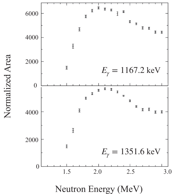
FIG. 1. Excitation functions for the 1431.4 keV level in ^{168}\text{Er} : plots of \gamma ray yields as a function of neutron energy. These plots show that two \gamma rays from the same level will demonstrate the same shape and energy threshold in the excitation function.
