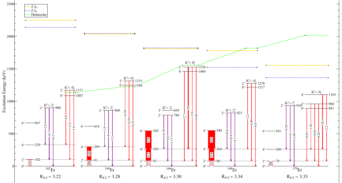
FIG. 5. Level schemes for ^{162-170}\text{Er} nuclei showing the depopulation and B(E2) values for the transitions from the first excited 0^+ and 2^+ bands. In green, we show the calculated energies [15] of the excited 0^+ state that is an oscillation on the ground state. In the dotted yellow and blue are the two-proton and two-neutron pairing gaps, respectively. The pairing gaps are calculated using the formulas in Ref. [40] and masses from Ref. [41].
