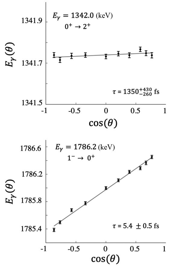
FIG. 3. Lifetime examples for ^{168}\text{Er}(n, n'\gamma) with a neutron energy of 2.0 MeV. The top figure is an example of the E_{\text{level}} = 1421.5 keV, 0^+_3 decay to 2^+_g , giving a new lifetime in this work. The bottom figure shows the lifetime of E_{\text{level}} = 1786.2 keV, 1^- decay to the ground state, which is in good agreement to the literature value of 5 \pm 1 fs.
