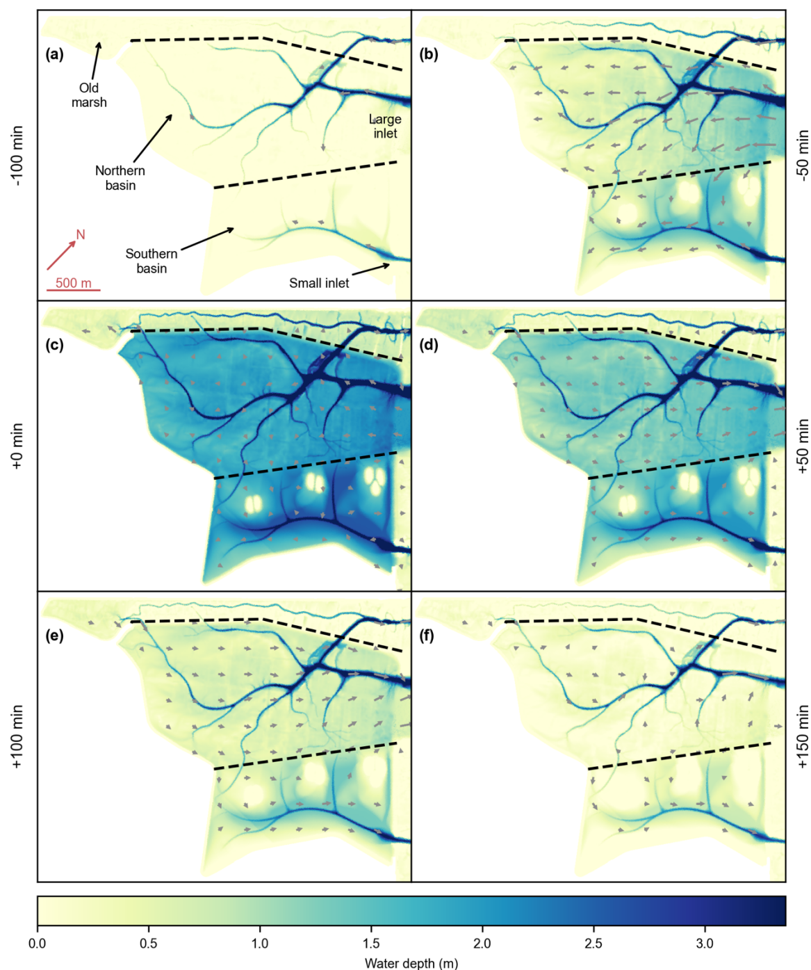
435 Figure 7: Reference model scenario (#1). Water depth (color maps) and flow velocity (grey arrows) every 50 minutes during a spring tide of the first year after de-embankment. Time tags are relative to high tide. Flow velocity arrows are not displayed if their magnitude is lower than 0.1 \text{ m s}^{-1} or if the water depth is lower than 10 cm. The dashed lines delineate the old marsh, the Northern basin, and the Southern basin. All figures are rotated by 43^\circ clockwise, as compared to Fig. 2c.
