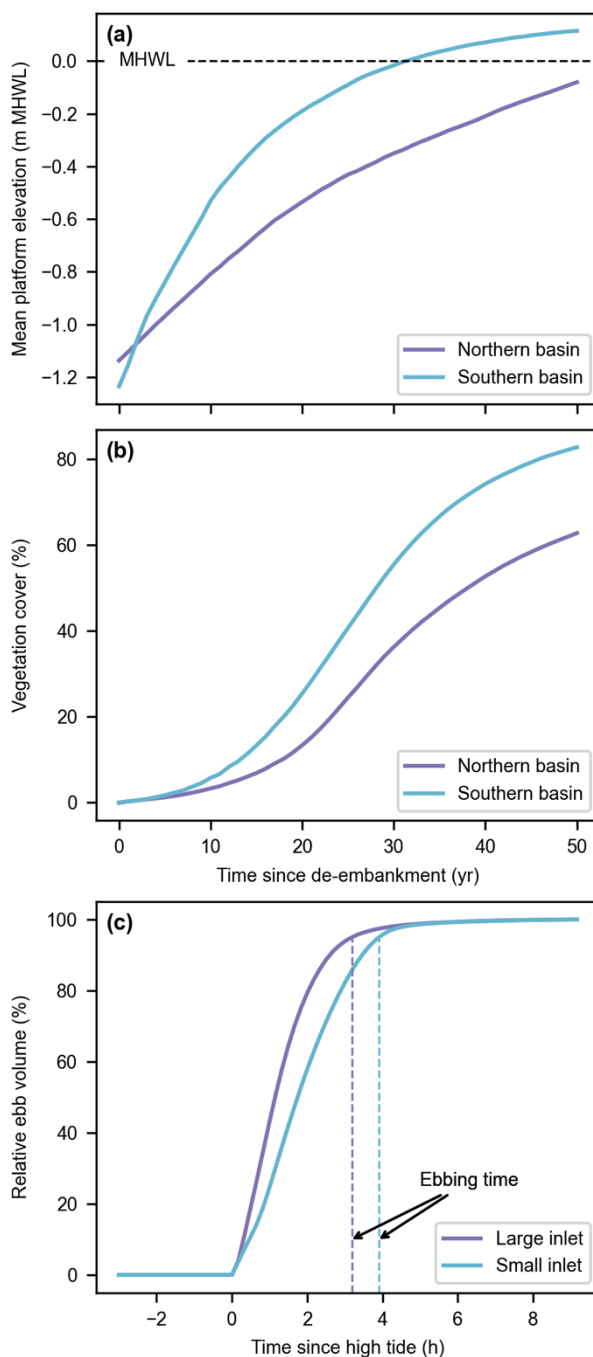
Figure 6: Reference model scenario (#1). Evolution of the mean platform elevation with respect to the mean high-water level (MHWL) (a) and development of the vegetation cover (b) in the Northern and Southern basins. Evolution of the relative ebb volume (i.e., the percentage of water volume flowing through an inlet since high tide during the ebb phase, see Sect. 2.5) and resulting ebbing time (i.e., the time corresponding to a relative ebb volume of 95%, proxy for inlet flush efficiency, see Sect. 2.5) for the large and small inlets during a spring tide of the first year after de-embankment (c).
