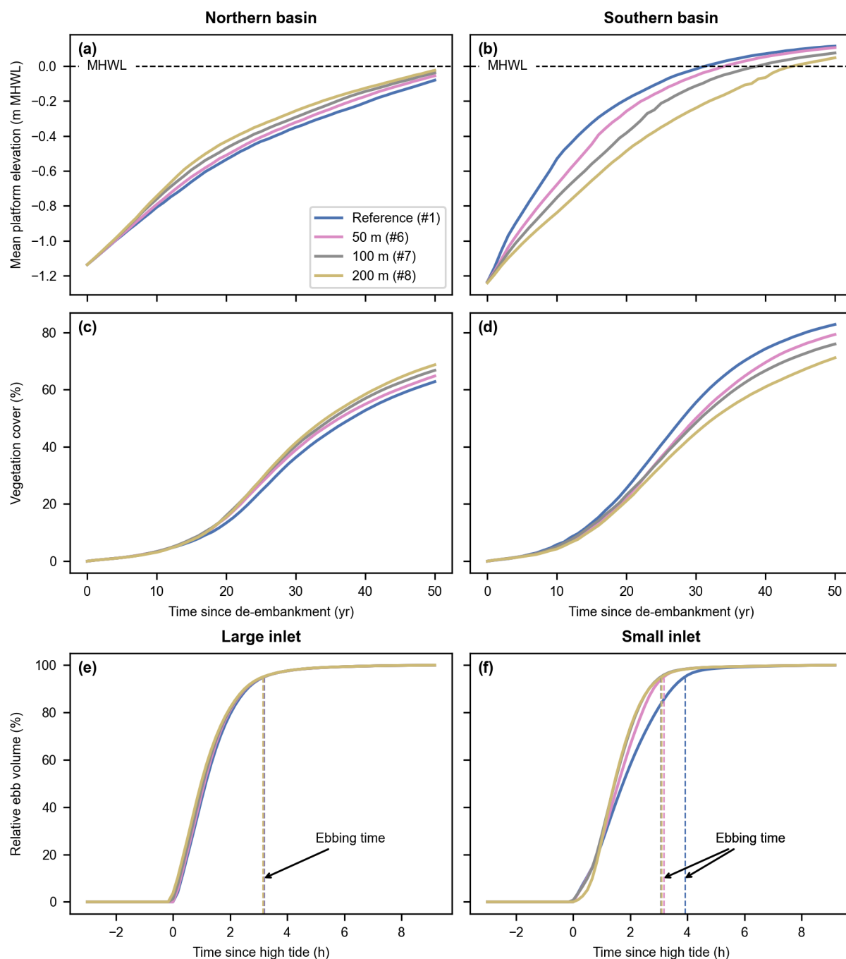
445 Figure 9: Inlet design model scenarios (i.e., reference design and three alternative designs with small-inlet widths of respectively 50, 100 and 200 m, and an excavated channel – #1, 6-8). Evolution of the mean platform elevation with respect to the mean high-water level (MHWL) (a-b) and development of the vegetation cover (c-d) in the Northern (a, c) and Southern basins (b, d). Evolution of the relative ebb volume (i.e., the percentage of water volume flowing through an inlet since high tide during the ebb phase, see Sect. 2.5) and resulting ebbing time (i.e., the time corresponding to a relative ebb volume of 95%, proxy for inlet flush efficiency, see Sect. 2.5) for the large (e) and small (f) inlets during a spring tide of the first year after de-embankment.
