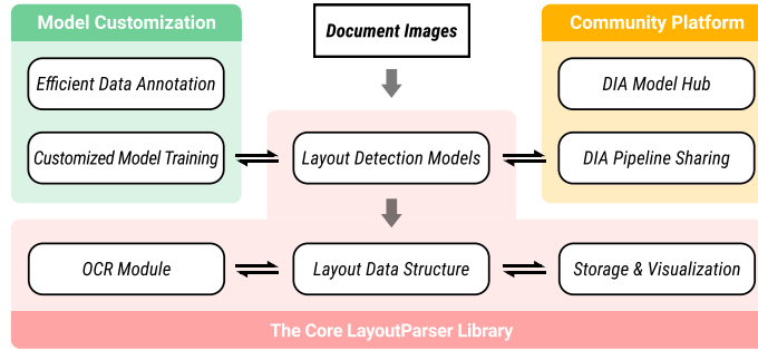
Fig. 1: The overall architecture of LayoutParser . For an input document image, the core LayoutParser library provides a set of off-the-shelf tools for layout detection, OCR, visualization, and storage, backed by a carefully designed layout data structure. LayoutParser also supports high level customization via efficient layout annotation and model training functions. These improve model accuracy on the target samples. The community platform enables the easy sharing of DIA models and whole digitization pipelines to promote reusability and reproducibility. A collection of detailed documentation, tutorials and exemplar projects make LayoutParser easy to learn and use.
