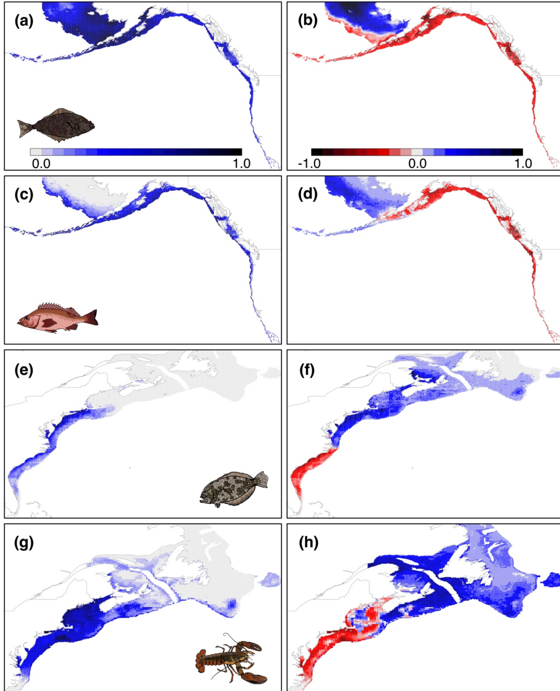
Figure 7. Ensemble mean projections across 18 Earth system models and 6 niche models for the RCP 8.5 scenario for Pacific halibut (a, b), Pacific ocean perch (c, d), summer flounder (e, f) and American lobster (g, h). For each species the left panel shows projected suitable habitat for the initial time period of 2007-2020, and the intensity of the blue represents habitat suitability while gray represents areas of the projection grid that are not suitable. The right panels show projected change in habitat suitability between the 2081-2100 time period and 2007-2020. For the right panels, red represents a decline in habitat suitability, blue represents increases in habitat suitability and gray represents areas of no change; increasing intensity of blue (red) represents a proportionally greater increase (decrease) in habitat suitability.
