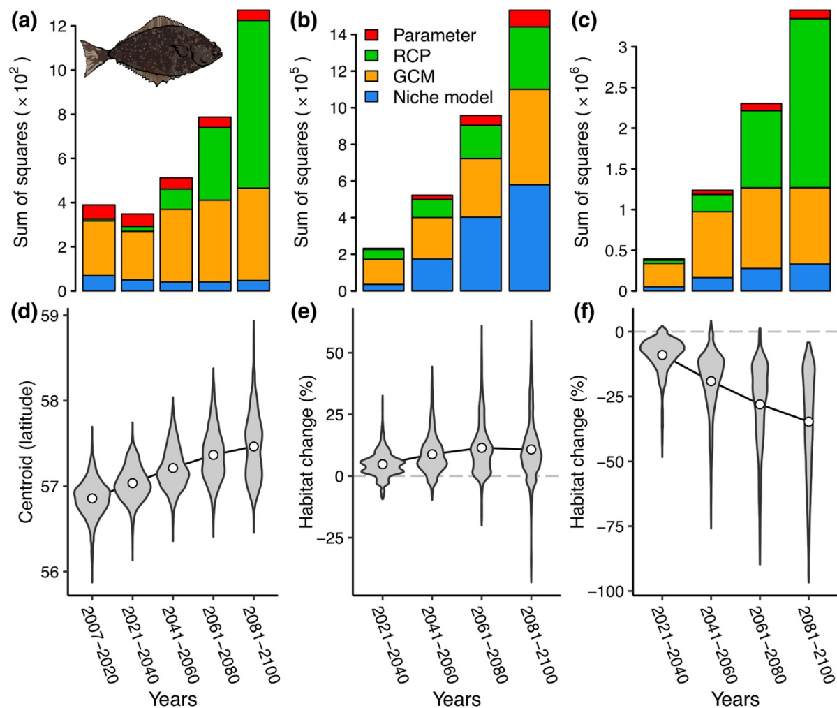
Figure 2. Sources of projection uncertainty for Pacific halibut Hippoglossus stenolepis . Partitioning of the sum of squares (a, b, c) with general linear models and distributions of projection results (d, e, f) by time period for latitudinal centroid (a, d), and percentage change in suitable habitat from the initial (2007-2020) time period for the northern region (b, e) and the southern region (c, f). Circles in d, e, and f are mean values.
