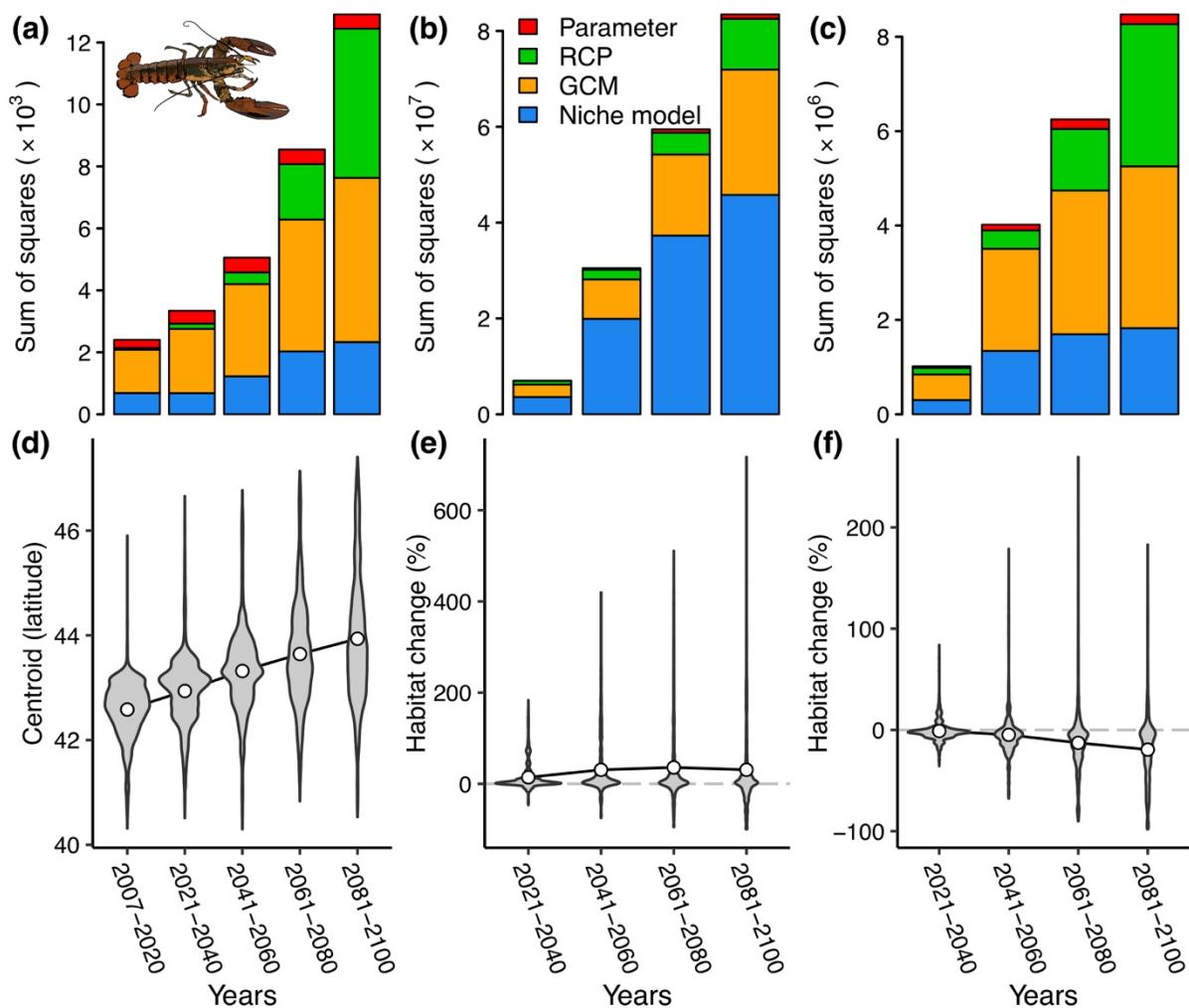
Figure 5. Sources of projection uncertainty for American lobster Homarus americanus . Partitioning of the sum of squares (a, b, c) with general linear models and distributions of projection results (d, e, f) by time period for latitudinal centroid (a, d), and percentage change in suitable habitat from the initial (2007-2020) time period for the northern region (b, e) and the southern region (c, f). Circles in d, e, and f are mean values.
