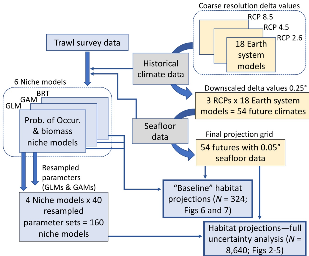
Figure 1. Modeling approach used for each species to project shifts in habitat suitability and to quantify uncertainty among niche modeling approach, parameter uncertainty within niche models, RCP climate scenario, and climate simulation model. Biological data and models are in blue, static and historical environmental data are in gray, and projected climate data are in yellow.
