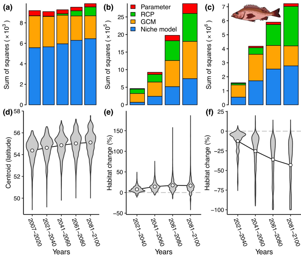
Figure 3. Sources of projection uncertainty for Pacific ocean perch Sebastes alutus . Partitioning of the sum of squares (a, b, c) with general linear models and distributions of projection results (d, e, f) by time period for latitudinal centroid (a, d), and percentage change in suitable habitat from the initial (2007-2020) time period for the northern region (b, e) and the southern region (c, f). Circles in d, e, and f are mean values.
