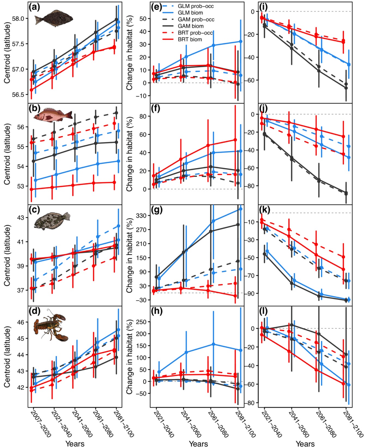
Figure 6. Ensemble mean projections for the RCP 8.5 scenario using six different niche models including generalized linear models (blue), generalized additive models (dark gray) and boosted regression trees (red) for probability of occurrence (dashed line) or for delta-biomass (solid line). Error bars are one standard deviation and represent uncertainty among 18 Earth system models. Columns represent mean latitudinal centroid (a, b, c, d), and percentage change in suitable habitat from the initial time period (2007-2020) in the northern (b, f, g, h) and southern (c, j, k, l) regions for Pacific halibut (a, e, i), Pacific ocean perch (b, f, j), summer flounder (c, g, k) and American lobster (d, h, l). Note that the full extent of error bars are not shown in g and l.
