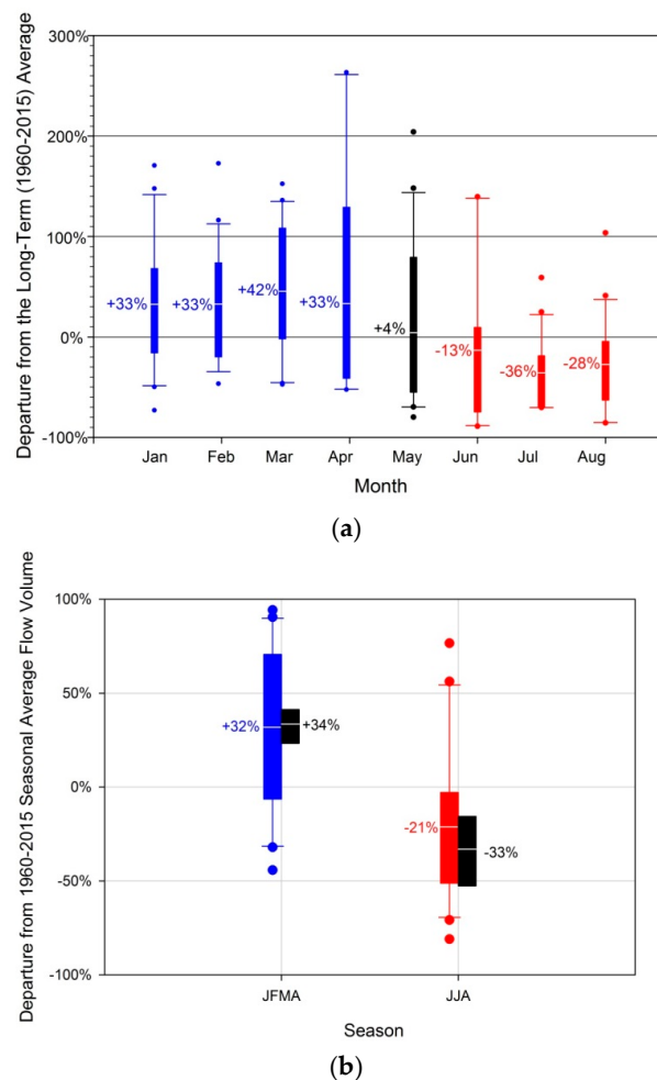
Figure 3. (a) Monthly departure (%) for post-El Niño year streamflow when compared to the long-term average for five gages in coastal MS-AL. (b) Seasonal (JFMA (blue) and JJA (red)) departure (%) for post-El Niño year streamflow when compared to the long-term average for five gages in coastal MS-AL and seasonal (JFMA (black) and JJA (black)) departure (%) for 2016 streamflow when compared to the historic long-term average for five gages in coastal MS-AL. The lower boundary of the solid box represents the 25th percentile while the upper boundary of the solid box represents the 75th percentile. The lower whisker represents the 10th percentile while the upper whisker represents the 90th percentile. Outliers are displayed as dots.
