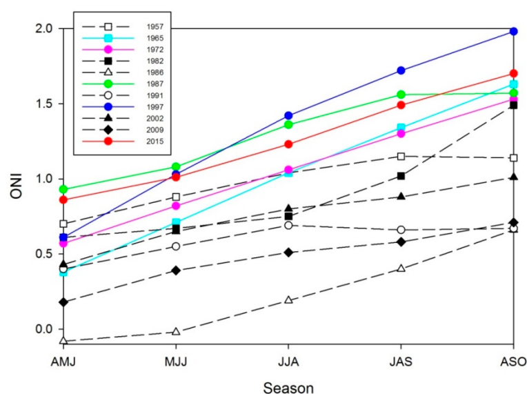
Figure 2. Recent (historic) and the 2015 observed El Niño events, based on Niño 3.4 sea surface temperature (SST) anomalies as quantified by the ONI. The x-axis shows three-month average (running mean) periods. Solid (colored) lines represent the four El Niño events similar to and the observed 2015 event. Dashed (black) lines represent dissimilar El Niño events.
