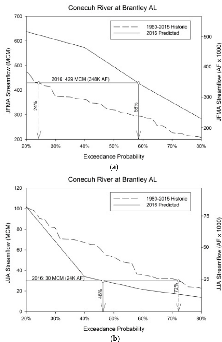
Figure 4. Observed (long-term average) and predicted (using historic El Niño events) exceedance probability curves for (a) winter-spring (JFMA) and (b) summer (JJA) seasonal streamflows for the Conecuh River. The observed 2016 streamflow for each season and corresponding exceedance probability is provided.
