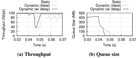
Figure 16: Effect of dynamic loop update
