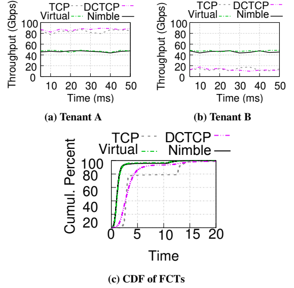
Figure 9: Performance isolation at scale
