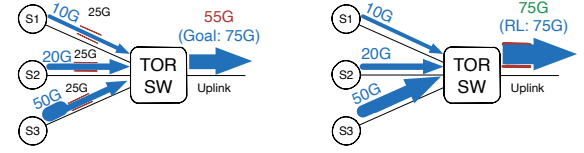
(a) Edge-based Rate-Limiting (b) In-network Rate-Limiting Figure 1: Example of how in-network rate-limiters can provide more precise rate-limiting and achieve higher network utilization than edge-based rate-limiters.
