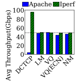
Figure 6: Data center applications
