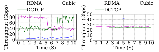
Figure 7: Experiment with Different Congestion Control Algorithms
