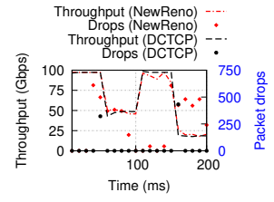
Figure 19: TCP friendliness
