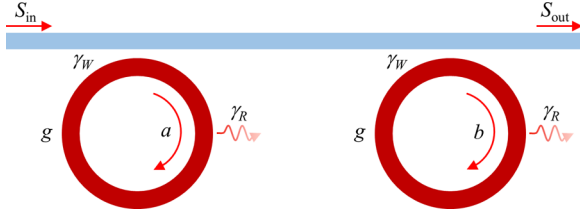
FIG. 4. Series of two identical optical amplifiers with CW modes a and b coupled through a common waveguide. Both resonators have the same gain g with identical coupling coefficients \gamma_W and radiation loss \gamma_R .
