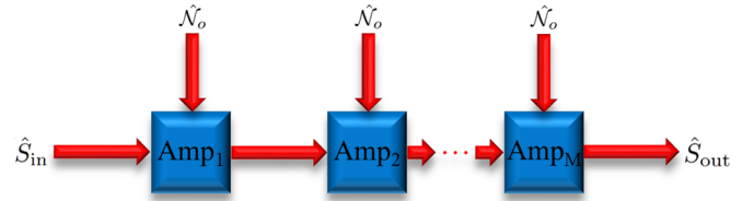
FIG. 7. Cascaded optical amplifier configuration with an EP of order M . An input signal \hat{S}_{\text{in}} from the leftmost waveguide enters amplifier \text{Amp}_1 that has quantum noise \hat{N}_o . The output of this amplifier is then fed into a second waveguide and then into a second amplifier that also has quantum noise \hat{N}_o , with this process then repeating for M amplifiers. For large values of gain, the noise of \text{Amp}_1 will dominate the quantum noise in \hat{S}_{\text{out}} .
