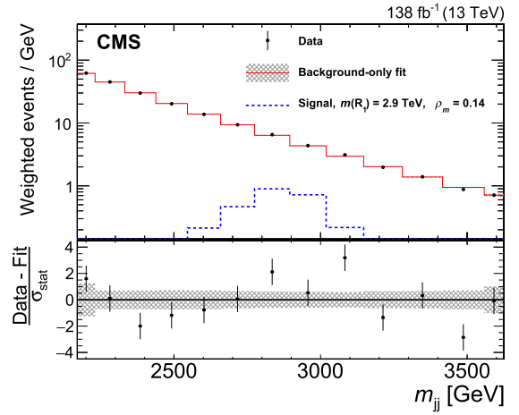
Fig. 4. Dijet mass spectrum, from the combination of the spectra within 22 categories, from the search for a resonance with mass m(R_1) = m(G_{KK}) = 2.9 TeV decaying to a second resonance with mass m(R_2) = m(\phi) = 0.4 TeV and a gluon. The figure shows the data (black points), the resulting background-only fit (solid line) and its uncertainty (barely visible gray hatched area), and the signal normalized to a cross section equal to the 95% CL observed limit (dashed line). The data shown in each bin are the weighted sum of the number of events within each category, divided by the bin width, as a function of the dijet mass, with vertical bars representing the statistical uncertainty ( \sigma_{stat} ). The weight of each event is equal to the fraction of signal events in the category to which it is assigned, assuming a signal cross section equal to the 95% CL observed upper limit. The same quantities are also shown for the background-only fits in each category, and for the signal. The lower panel shows the difference between the data and the background prediction (points), and the background uncertainty (hatched gray area), divided by the statistical uncertainty.
