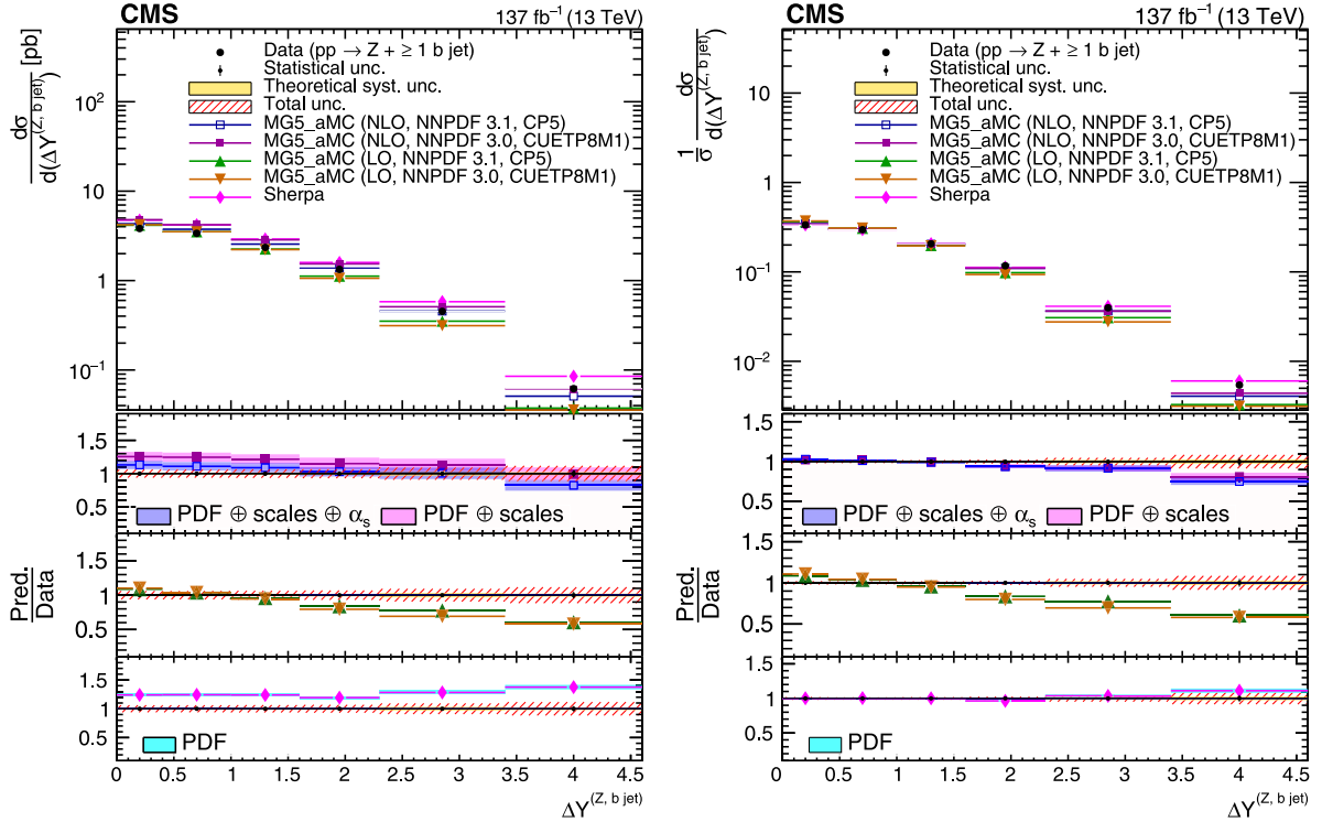
FIG. 6. (left) Differential cross section and the (right) normalized differential cross section distributions as functions of \Delta Y^{(Z, b \text{ jet})} between the Z boson and the leading b jet for the Z + \geq 1 b jet events.
