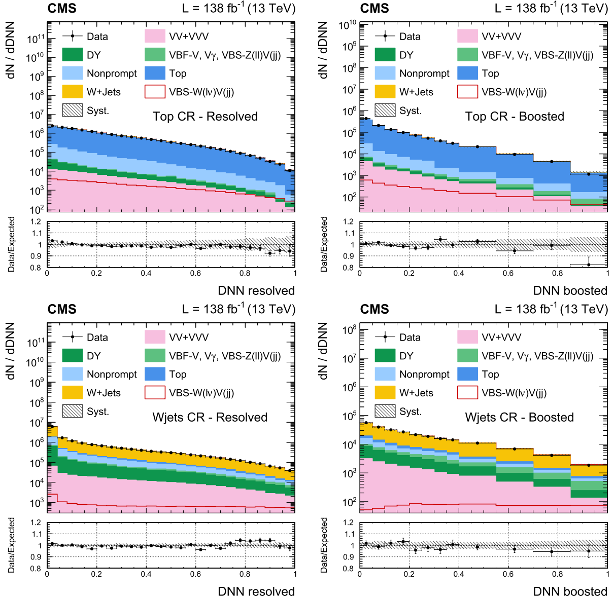
Fig. 4. The DNN discriminator distribution for the resolved (left) and boosted (right) phase space region in the top quark (upper plots) and W+jets (lower plots) control regions. Vertical bars on data points show the statistical error, whereas the gray band is the post-fit uncertainty on MC with all systematic uncertainties included.
