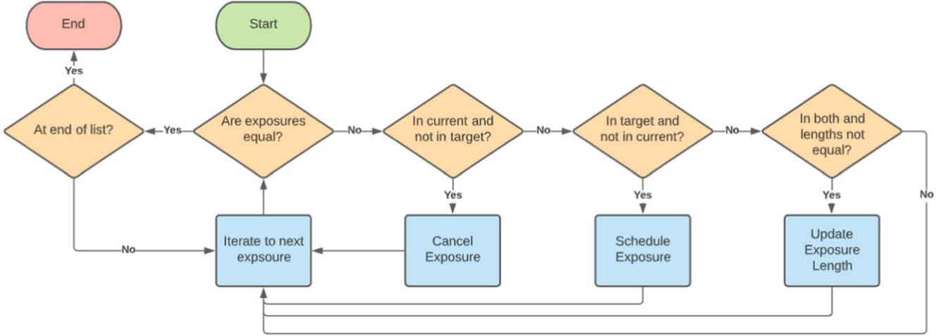
Figure 3. The matching algorithm comprising of the CM’s third and forth main objectives as described in Section 4.1. Following the generation of the current list, i.e., the list of currently scheduled exposures, and the target list, i.e., the list of exposures that should be scheduled based on any recent user-inputted changes, the CM iterates through both lists, compares their properties, and modifies the current list to match the target list.
