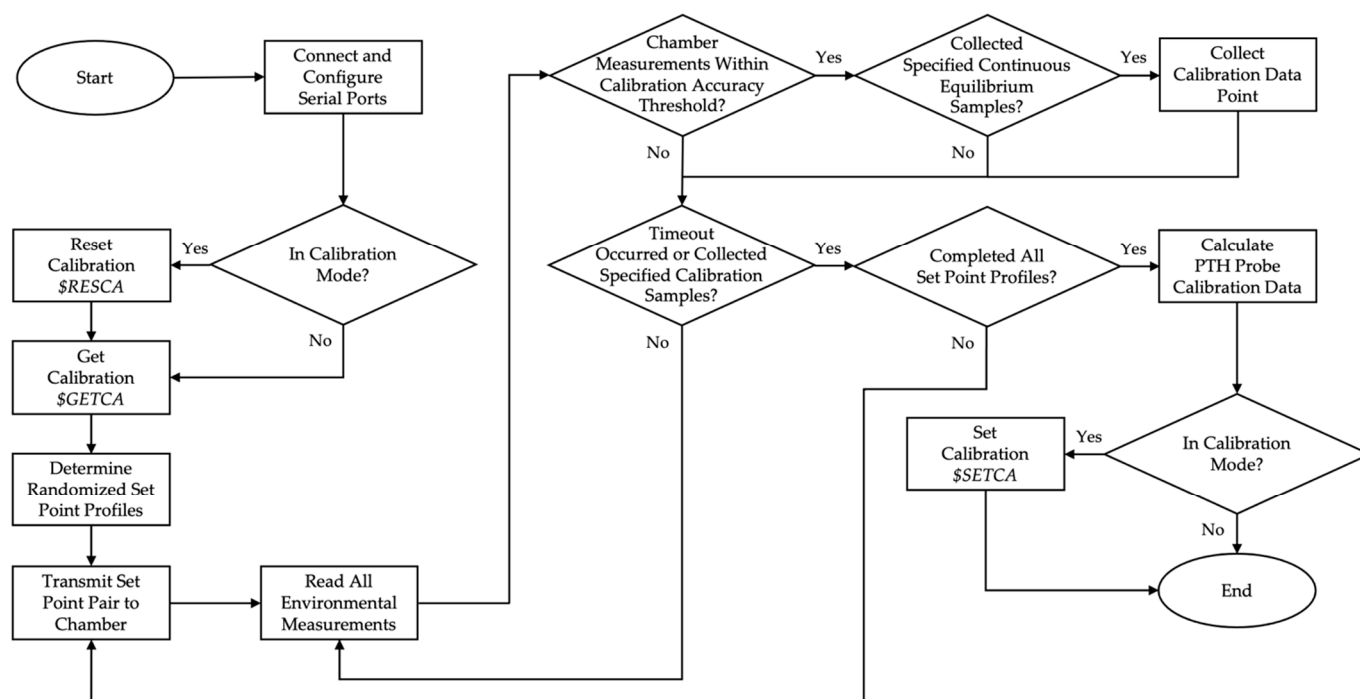
Figure 6. Block diagram of the automated calibration system generalizing functionality.
