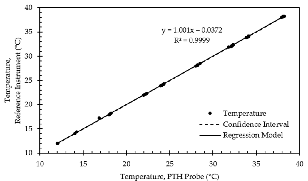
Figure 15. Regression model and corresponding confidence interval for temperature validation data from representative PTH probe (SN: 0x0005).
