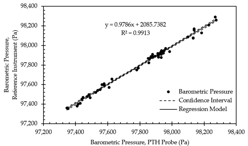
Figure 14. Regression model and corresponding confidence interval for barometric pressure validation data from representative PTH probe (SN: 0x0005).
