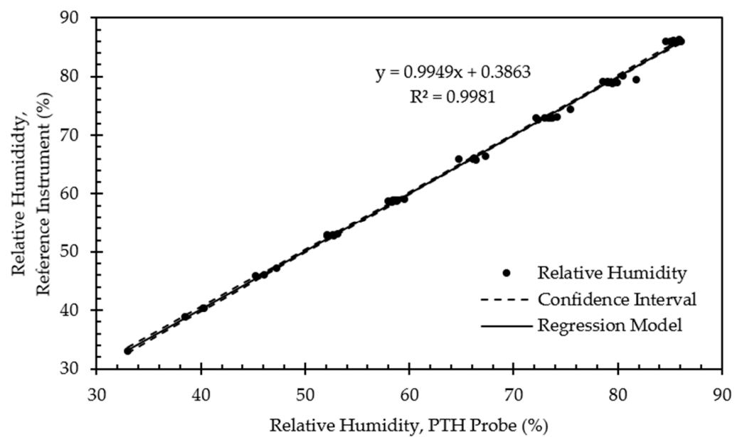
Figure 16. Regression model and corresponding confidence interval for relative humidity validation data from representative PTH probe (SN: 0x0005).
