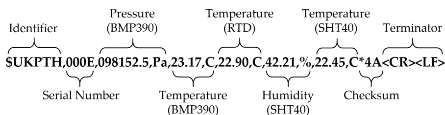
Figure 3. Example formatted string transmitted from the PTH probe to the host at 1 Hz over 3.3 VDC TTL UART. The checksum was the bit-wise exclusive OR of all 8-bit ASCII characters between the '$' and '*' characters and displayed as a 2-digit hexadecimal number. The terminator comprised the non-printable carriage return <CR> and line feed <LF> characters.
