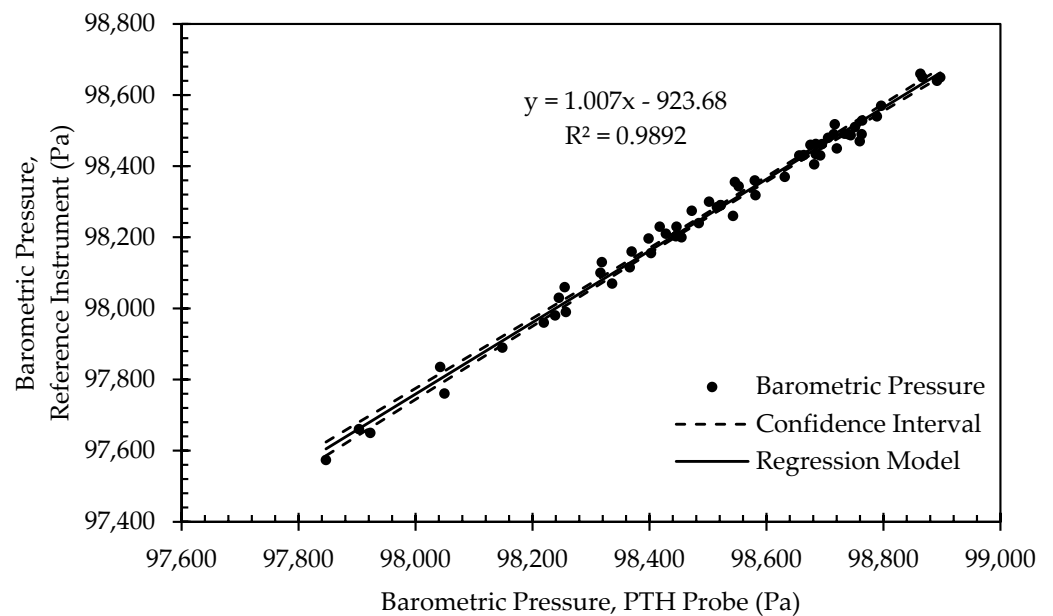
Figure 10. Regression model and corresponding confidence interval for barometric pressure calibration data from representative PTH probe (SN: 0x0005).
