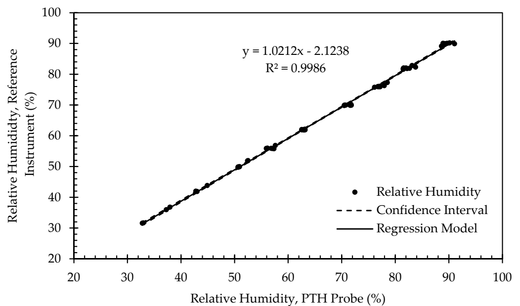
Figure 12. Regression model and corresponding confidence interval for relative humidity calibration data from representative PTH probe (SN: 0x0005).
