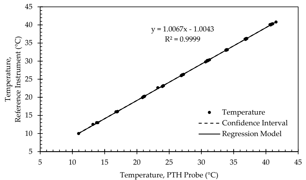
Figure 11. Regression model and corresponding confidence interval for temperature calibration data from representative PTH probe (SN: 0x0005).
