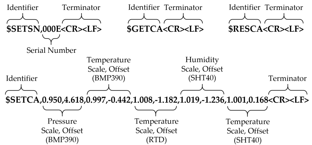
Figure 4. Example formatted strings received by the PTH probe from the host over 3.3 VDC TTL UART. The PTH probe responded by echoing the string with relevant data and checksum inserted before the terminator.
