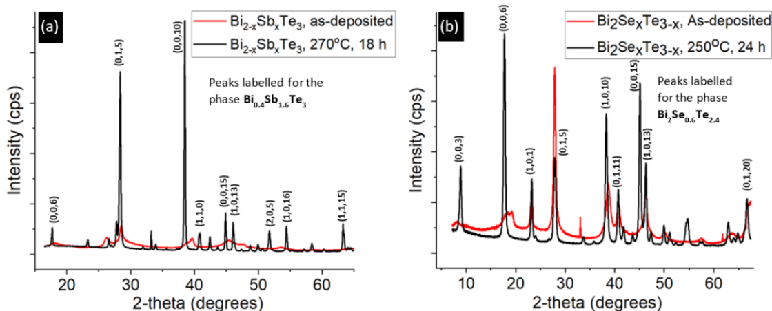
Figure 3. XRD data before and after post-deposition annealing. (a) P-type thin film sample demonstrates that baking at 270 °C for 18 h is essential for improving the crystallinity of the as-deposited film. (b) A similar change in crystallinity was observed on an n-type sample baked at 250 °C for 24 h.
