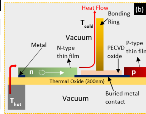
Figure 11. (a) Table showing the parameters used for the thermoelectric thin film deposition after optimization. (b) Cross-sectional schematic view of a hybrid heat flow planar TEG excluding the top and bottom headers.
