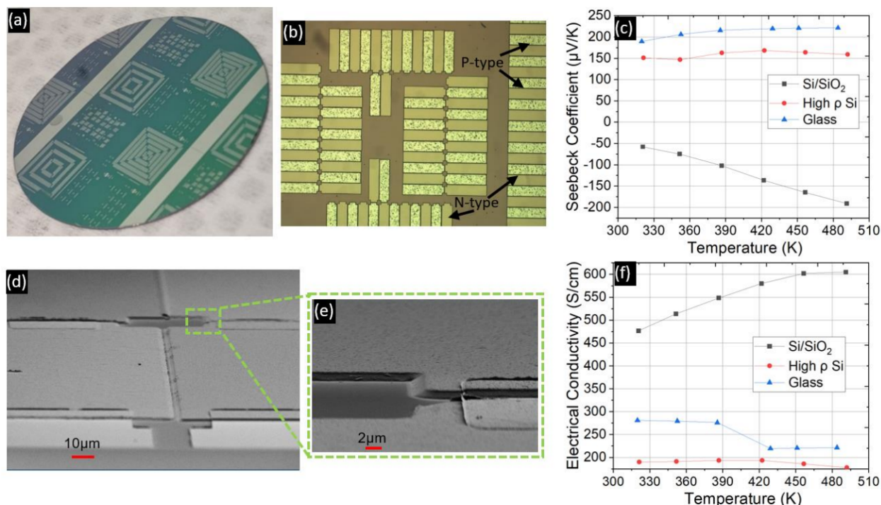
Figure 9. (a) Successful lift-off of p-type and n-type thin films on a 2" Si/SiO 2 wafer. N-type thin films were deposited before p-type, requiring a higher post-deposition bake temperature. A 15 nm Cr adhesion layer was deposited in situ before the thermoelectric thin film evaporation. (b) Zoomed-in view of the wafer from (a). (c) Negative Seebeck coefficients were measured on a Si/SiO 2 substrate where a Cr adhesion layer was deposited before evaporation of the pellets. The data with a positive Seebeck coefficient corresponds to samples loaded during the same run but on glass and high resistivity (ρ) Si substrates. (f) Corresponding electrical conductivity data. (d) SEM images showing the thermocouples displayed in (a,b). Ni contacts deposited over the thermoelectric thin films to form test structures are also visible (e) The zoomed-in view shows the slope of the thermoelectric thin films indicating that the rotation of the wafer can distort the boundary of the features and highlighting the importance of a large undercut during the lithography.
