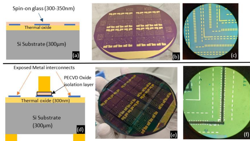
Figure 12. (a) Schematic view of the wafer at the end of Stage 1. (b) 4" wafer after Stage 1 with Ti/Ni/Au interconnects. (c) Zoomed-in view of the interconnects. (d) Schematic view after Stage 2 of fabrication. (e) Wafer-level view post Stage 2 after completing bonding ring formation on both sides of the wafer followed by etching of the PECVD oxide to reveal the metal interconnects. (f) Zoomed-in top view of the wafer at the end of Stage 2.
