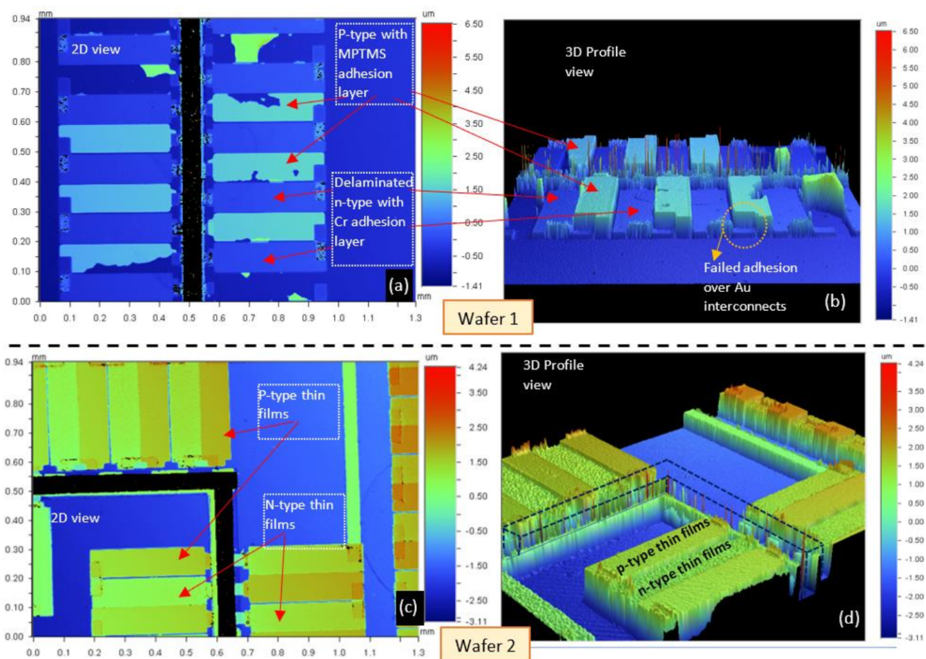
Figure 14. (a) 2D view of a section on W1 depicting the failed lift-off of n-type thin films having a Cr adhesion layer and the partially failed lift-off of p-type thin films with MPTMS adhesion layer (b) 3D profiles created from (a) that highlight the lack of adhesion between p-type thin films and the interconnects. In the n-type areas, only the Cr adhesion layer is left. (c) 2D view of a section on W2 displaying the thermoelectric thin films showing the p-type and n-type thin films, metal contacts, and the bonding ring. (d) 3D view created from the optical profilometry data measured in (a). The dashed lines are drawn to indicate the bonding ring as the profilometry tool could not focus on the top of the Au bonding ring surface.
