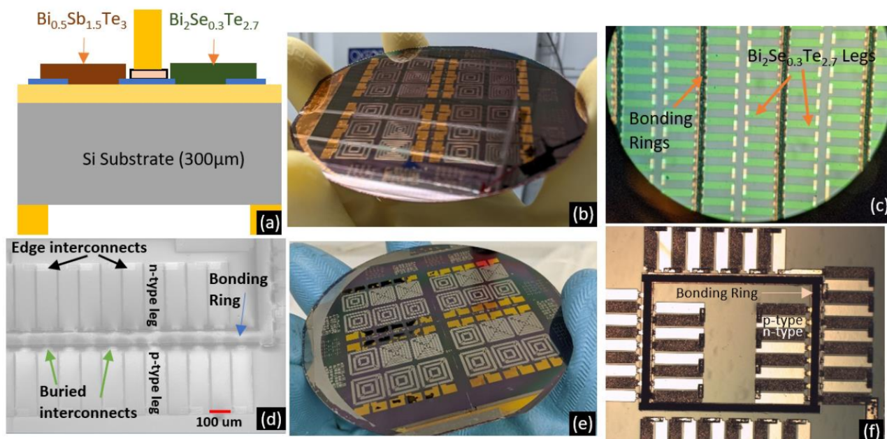
Figure 13. (a) Schematic view of the cross-section of one thermocouple after Stage 3 of fabrication. (b) Wafer view after evaporation and lift-off of n-type thin films. (c) Zoomed-in view of n-type thin films. (d) SEM image of a section of a single device after deposition of both p-type and n-type thermoelectric thin films. (e) Wafer view after both rounds of deposition. (f) Zoomed-in picture of a section of the device.
