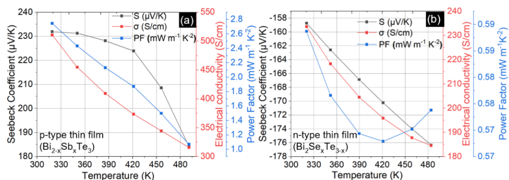
Figure 4. Thermoelectric properties versus temperatures for p-type (a) and n-type (b) films deposited on glass substrates. Amongst the samples we synthesized, these films had the highest power factor near room temperature.
