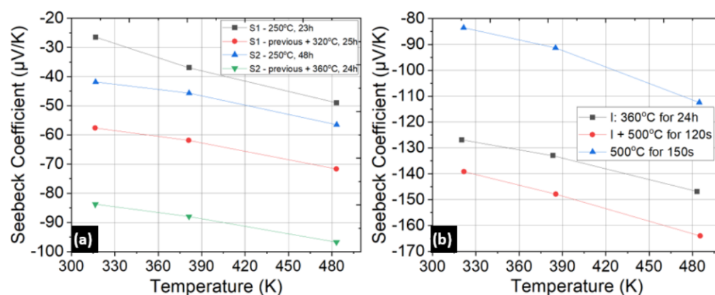
Figure 7. (a) Increase in the Seebeck coefficient of n-type Se 12 xTe 1 x thin films seen upon long bakes at higher temperatures of 320 °C (Sample 1 → S1) and 360 °C (Sample 2 → S2). (b) Seebeck coefficients of the optimum thin films obtained from pellet composition of Se 9 xTe 2 x, and a high-temperature bake at 360 °C. Short-term high heat treatment at 500 °C showed improvement but was also seen to damage the surface of one of the samples; hence, it was excluded from the subsequent batches.
