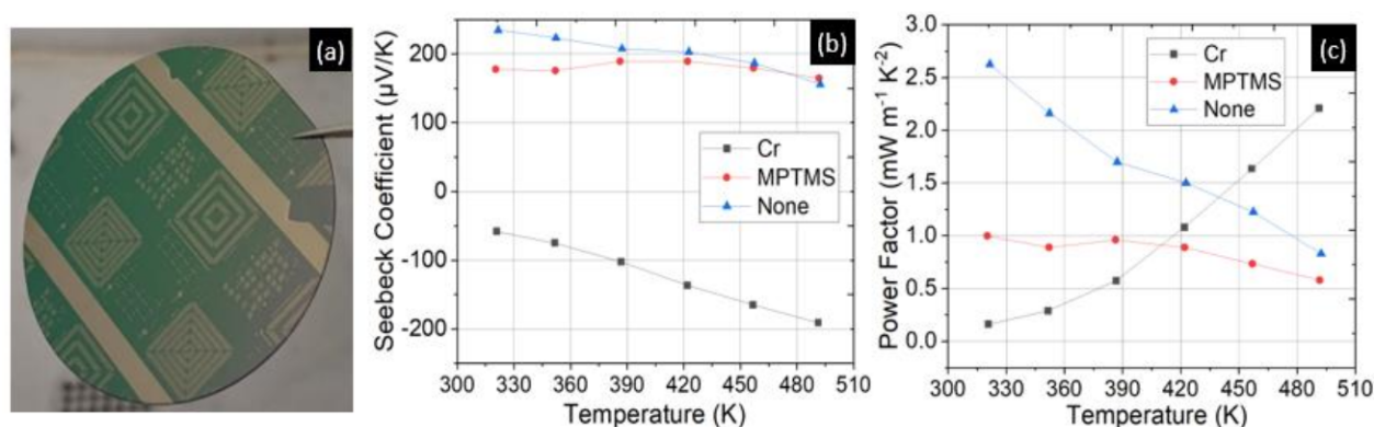
Figure 10. (a) Successful lift-off on a Si/SiO 2 substrate after deposition of p-type thin films. (b,c) Comparison of thermoelectric data measured on Si/SiO 2 substrates from runs 1r, 1s, and 1t from Table 3 with the adhesion layers as stated in the legend. Application of MPTMS resolved the negative Seebeck data issue while facilitating lift-off of p-type thin films.
