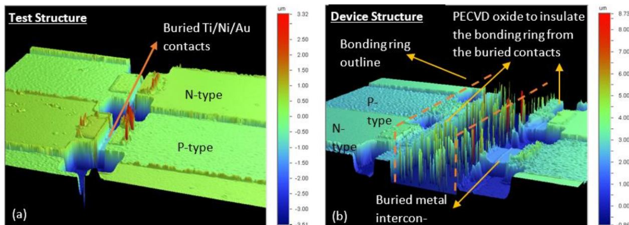
Figure 15. (a) 3D profile of a test structure without a bonding ring between each thermocouple-like structure. (b) The device structure's 3D profile illustrates the PECVD oxide on which the bonding ring is deposited to insulate it from the buried metal interconnects connecting the thin films on either side of the bonding ring.
