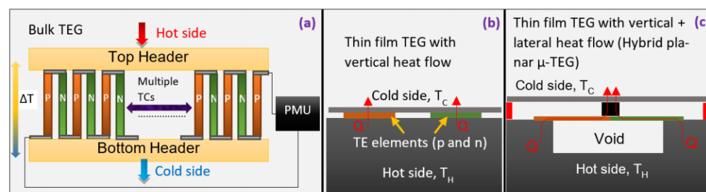
Figure 1. (a) Conventional bulk TEG design with p-type and n-type thermoelectric legs placed between two headers. (b) A thin film TEG with vertical heat flow. (c) A thin film TEG with vertical and lateral heat flow, classified as a hybrid planar TEG.
