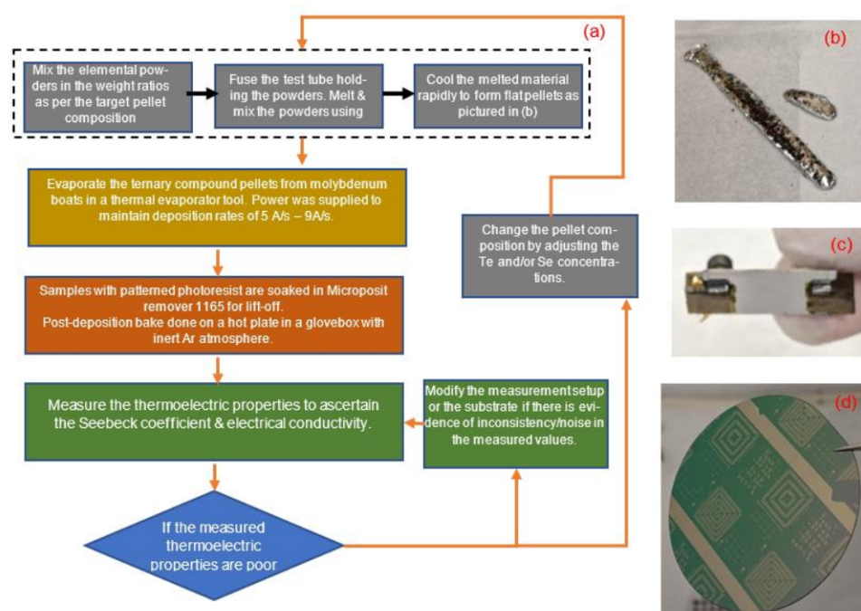
Figure 2. (a) The flowchart details the steps to achieve device-quality thin films. The composition of the ternary compound pellets and the post-deposition anneal were the key parameters explored for
