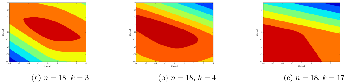
Fig 7: Contour plots of the estimated edge-triangle DERGM likelihood functions for the Sampson network, for various values of (\theta_1, \theta_2) . Here, n = 18 and k = 3, 4, 17 . Note that k = 17 corresponds to the full ERGM. The estimated likelihood is based on an iid sample of 25,000 graphs in \mathcal{G}_{n,k} .
