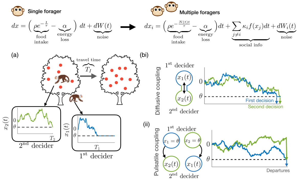
FIG. 1. Evidence accumulation model for patch leaving in individuals and groups. (a) Schematic of patch departure decision in a group with two agents. (b) (i) Diffusive coupling —agents communicate their beliefs throughout the evidence accumulation process to their neighbors. (ii) Pulsatile coupling —agents only communicate their decision to leave the patch to their neighbors.
