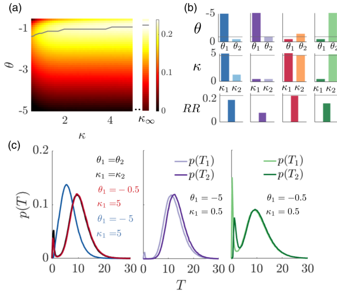
FIG. 3. Comparison of reward rates (RRs) in a group with diffusively coupled belief states. (a) Heat map shows how reward rate varies with the decision threshold \theta and coupling strength \kappa for a symmetric model \theta_1 = \theta_2 = \theta and \kappa_1 = \kappa_2 = \kappa , and \alpha = 1 , \rho = 4 , \tau = 5 , and T_l = 5 . Decision and departure time statistics are obtained by running Monte Carlo simulations for Eq. (2) (see Appendix A 2 a). Grey line: Optimal threshold value \theta^{\text{opt}} for fixed coupling strength. The line is smoothed by computing averages over a sliding window of length 3. Right column: RR for the infinite coupling limit ( \kappa \rightarrow \infty ). (b) Asymmetric strategies. Optimal threshold \theta_2 (1st row), coupling \kappa_2 (2nd row), and RR (3rd row) when fixing agent 1 threshold \theta_1 and coupling strength \kappa_1 . Grey line: Optimal symmetric \theta and \kappa . (c) Patch departure decision time distributions for each group in (b).
