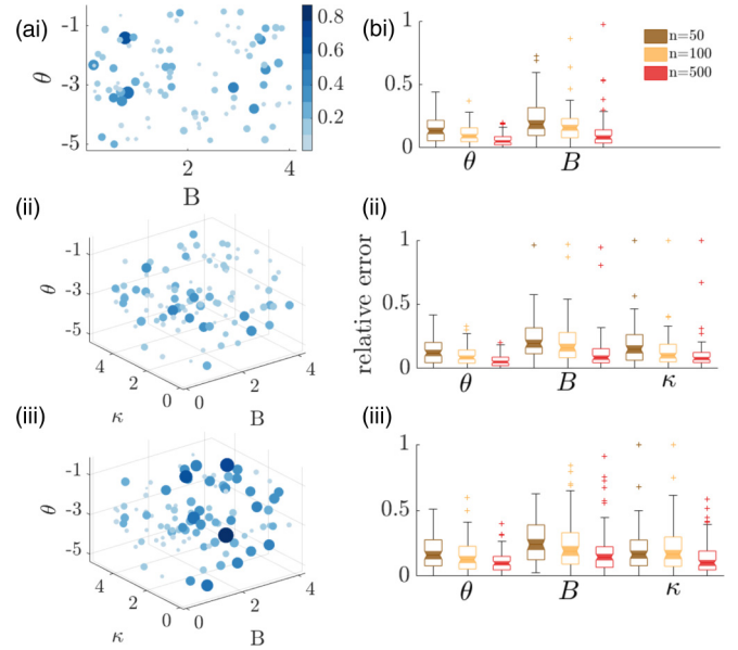
FIG. 5. Parametric fits of no coupling, diffusive, and pulsatile model using Bayesian maximum a posteriori (MAP) estimation. (a) Estimation errors for (i) no information coupling, (ii) diffusive coupling, and (iii) pulsatile coupling. Bubble location represents true parameters and bubble size/color indicates the total sum of relative estimation error for displayed parameters, Eq. (7). Each plot is obtained from 100 parametric samples from a uniform prior where \theta \in [-0.1, -5] , \kappa \in [0.1, 6] , B \in [0.1, 4] given n = 100 departure time samples each. (b) Box plots showing the median relative error (notches), upper/lower quartiles (boxes), minimum/maximum excluding the outliers (error bars), and outliers (stars) in MAP estimate of the model parameters (\theta, B, \kappa) for (i) no information coupling, (ii) diffusive coupling, and (iii) pulsatile coupling models, calculated using data of sample size n = 50, 100, 500 . The displayed distributions of the relative error were computed using 100 parametric samples from a uniform prior.
