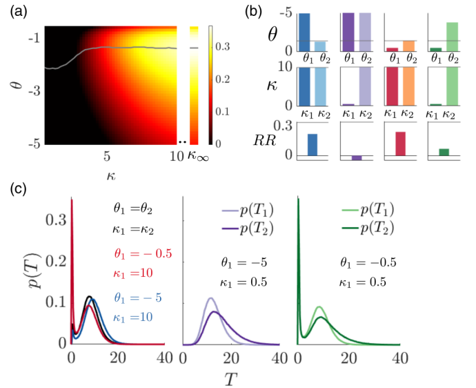
FIG. 4. Comparison of RRs in group with pulsatile coupling. (a) RR heat map for a two agent group with the same decision threshold \theta and coupling strength \kappa , and \alpha = 1 , \rho = 4 , \tau = 5 , and T_l = 5 . Decision and departure time statistics are obtained by running Monte Carlo simulations for Eq. (4) (see Appendix A 2 a). Grey line: Optimal decision threshold \theta for a given coupling strength. The line is smoothed by computing average over a sliding window of length 3. Right column: RR in the infinite coupling limit ( \kappa \rightarrow \infty ). (b) Asymmetric strategies. Optimal threshold \theta_2 (1st row), coupling \kappa_2 (2nd row), and RR (3rd row) for fixed agent 1 threshold \theta_1 and coupling strength \kappa_1 . Grey line: Optimal symmetric \theta and \kappa . (c) Patch departure decision time distributions for each group in (b).
