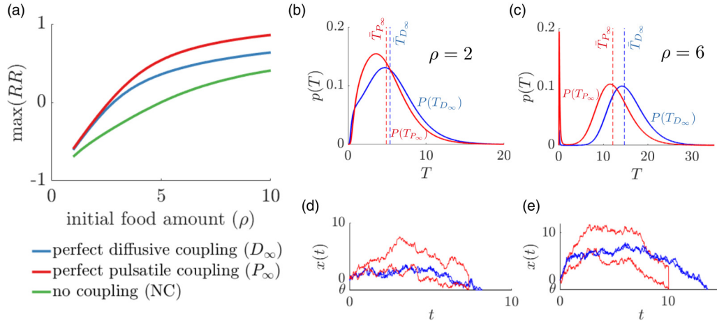
FIG. 2. Coupling of belief states between group members increases the reward rate (RR). (a) Comparison of reward rate for a two-agent system: perfectly diffusively coupled ( D_\infty ), perfectly pulsatile coupled ( P_\infty ), and no information coupling (NC). For lower values of initial food, diffusive and pulsatile coupling perform similarly generating higher reward compared to the uncoupled case. When the initial food amount is higher, pulsatile coupling outperforms diffusive coupling. For fixed values of model parameters \tau = 5 , B = 1 , \alpha = 1 , T_l = 5 , and \rho = 2 , we maximize the reward rate for the group by optimizing the patch departure threshold \theta . [(b),(c)] Patch departure time distribution for diffusive (blue) and pulsatile (red) coupling. The dashed line shows average patch departure time. A single simulation of pulsatile (red) and diffusive coupled (blue) models when (d) \rho = 2 and (e) \rho = 6 .
