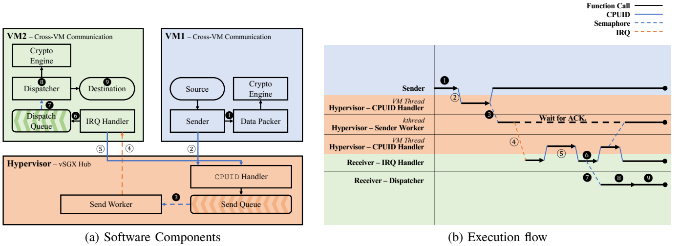
Fig. 4: Cross-VM communication.
