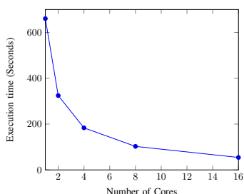
Fig. 6: Relation between execution time and number of available processing cores.
