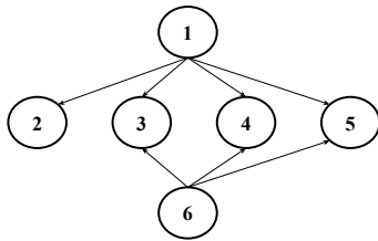
(c) Knowledge of mappings from the above code snippet with satisfying dependency and its graph.
