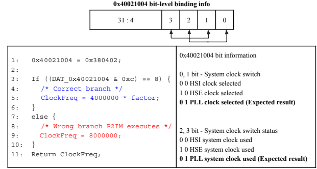
Figure 2: Simplified Real-world firmware code snippet where P2IM models a peripheral register in a wrong way.
