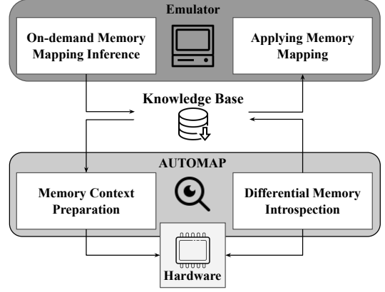
Figure 4: Overview of AUTOMAP.
