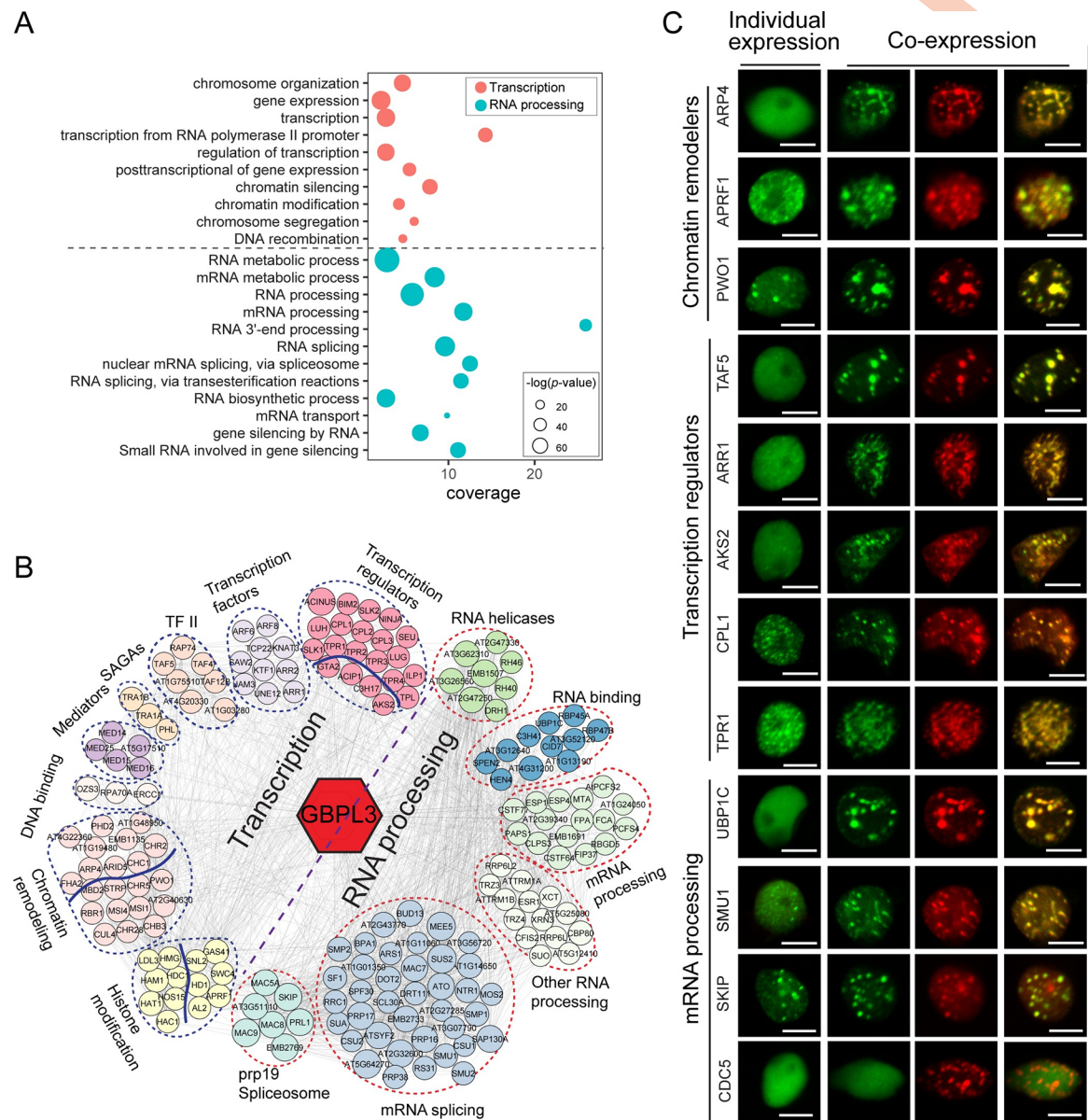
Fig 3. GBPL3 is capable of recruiting transcription regulators and RNA processing machinery. (A) GO enrichment analysis of GBPL3 proximate. GO terms under the 2 major molecular functions identified (transcription and RNA processing) are presented in a bubble plot. Underlying data can be found in S5 Data . (B) GBPL3 PPI network that contains 177 GBPL3 proximal proteins involved in transcription and RNA processing identified in (A). Cytoscape was used to construct and visualize the GBPL3 PPI network. GBPL3 interactors were clustered and color-coded manually based on published protein functions. Node sizes represent scores of PPIs retrieved from the STRING database ( https://string-db.org/ ). (C) Transient expression of selected GBPL3 proximal proteins involved in transcription regulation and RNA processing in N. benthamiana . The left column shows the individual expression of GFP-tagged GBPL3 proximal proteins, and the right 3 columns show coexpression with mCherry-GBPL3. CELL DIVISION CYCLE (CDC5), a putative TF, was included as a negative control. Bars = 10 μm. GO, gene ontology; PPI, protein–protein interaction; TF, transcription factor.
