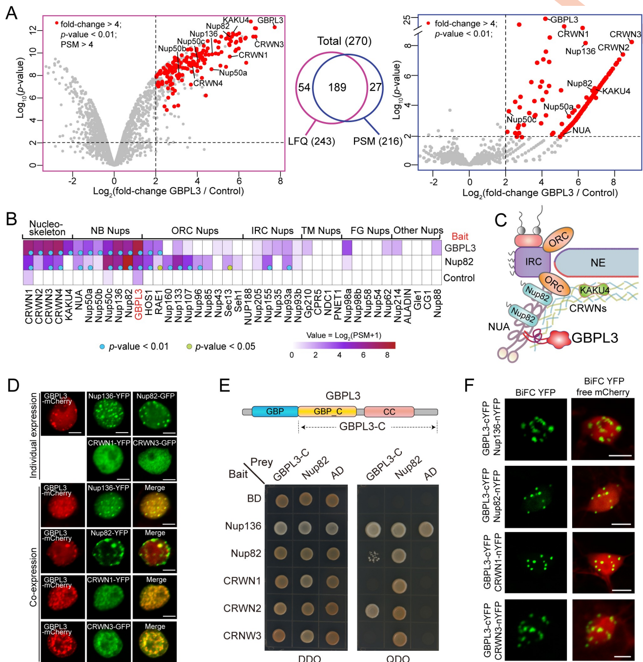
Fig 2. GBPL3 physically interacts with NPC basket and nucleoskeleton components. (A) Volcano plots of candidates identified by proximity labeling proteomics using GBPL3 as bait. Analyses based on the LFQ intensity and PSM data are shown on the left and right sides, respectively. The overlap of candidates identified by both analyses is shown in the middle. Non-transformants (WT) treated with biotin were used as control, and 2 biological replicates are included in the analysis. Significantly enriched proteins were selected using PSM > 4, fold-change > 4, and p-value < 0.01 as cutoffs and represented by red dots. The nuclear basket and nucleoskeleton components were text labeled. Underlying data can be found in S5 Data . (B) Heatmap showing normalized and averaged PSM values of all nucleoskeleton and nucleoporin proteins identified by GBPL3, Nup82, and KAKU4 using proximity labeling proteomics. Blue and green dots indicate p-value < 0.01 and 0.05, respectively. Nup82 and KAKU4 data were retrieved from PXD015919 and PXD026924, respectively. (C) A model diagram showing that the nuclear basket and the nucleoskeleton comprise a protein meshwork underneath the NPC and the position of GBPL3 at a more distal region of the NB. (D) Transient protein expression of GBPL3 and NPC basket components Nup136/ Nup82 and nucleoskeleton components CRWN1/CRWN3 in N. benthamiana . The upper 2 panels show individual protein expression, and the lower 4 panels show mCherry-GBPL3 coexpression with CRWN1-YFP, CRWN1-GFP, Nup136-YFP, or Nup82-GFP. Bars = 10 μm. (E) Yeast-two-hybrid analysis using GBPL3-C (GBP_C domain and IDRs) and Nup82 as the bait and Nup136, Nup82, CRWN1, CRWN2, CRWN3 as the prey. Zygote yeasts were
