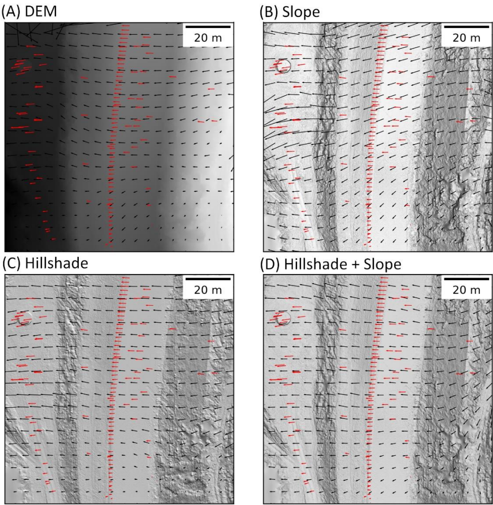
Figure 4. Visualization of the output 3D landslide displacement using 4 different DEM representations: (A) Normalized DEM, (B) Slope, (C) Hillshade, and (D) Combined Hillshade and slope. Black vectors show the output 2D displacement vectors plotted every 100 cells, while the red vectors show the ground truth vectors measured from the ground truth dataset. All vectors are scaled 20×.
