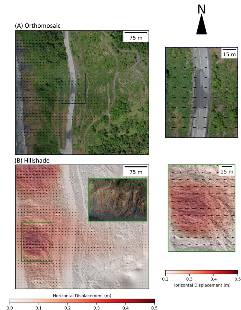
Figure 8. Visualization of the Horizontal displacement computed using SlideSim on the UAS data over the larger extents. Vectors are scaled 20×.
