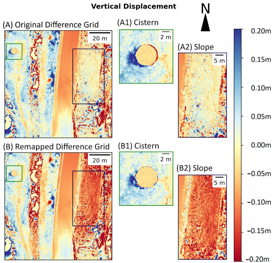
Figure 7. Vertical difference grid between DEMs from subsequent survey epochs from (A) a regular difference grid and (B) computed using the proposed remapping approach with close-up views of the cistern (#1) and hillslope (#2).
