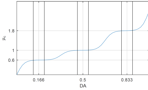
(a) Neuromodulatory factor \mu_c(DA) of receptor D2
