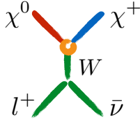
Figure 13: Left: Co-scattering efficient for dark matter produced in association with soft displaced b-jets at the LHC. Right: Dark matter produced in association with soft displaced leptons at the LHC.
