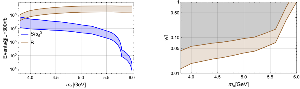
Figure 11: Signal (M1) and background expected number of events after selections for 300 fb -1 . The error bands for the background are taken from [154] and for the signal it is estimated by a 7-point renormalization and factorization scale dependence. Right : Estimated exclusion region on v/f .
