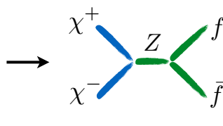
Figure 13: Left: Co-scattering efficient for dark matter produced in association with soft displaced b-jets at the LHC. Right: Dark matter produced in association with soft displaced leptons at the LHC.
