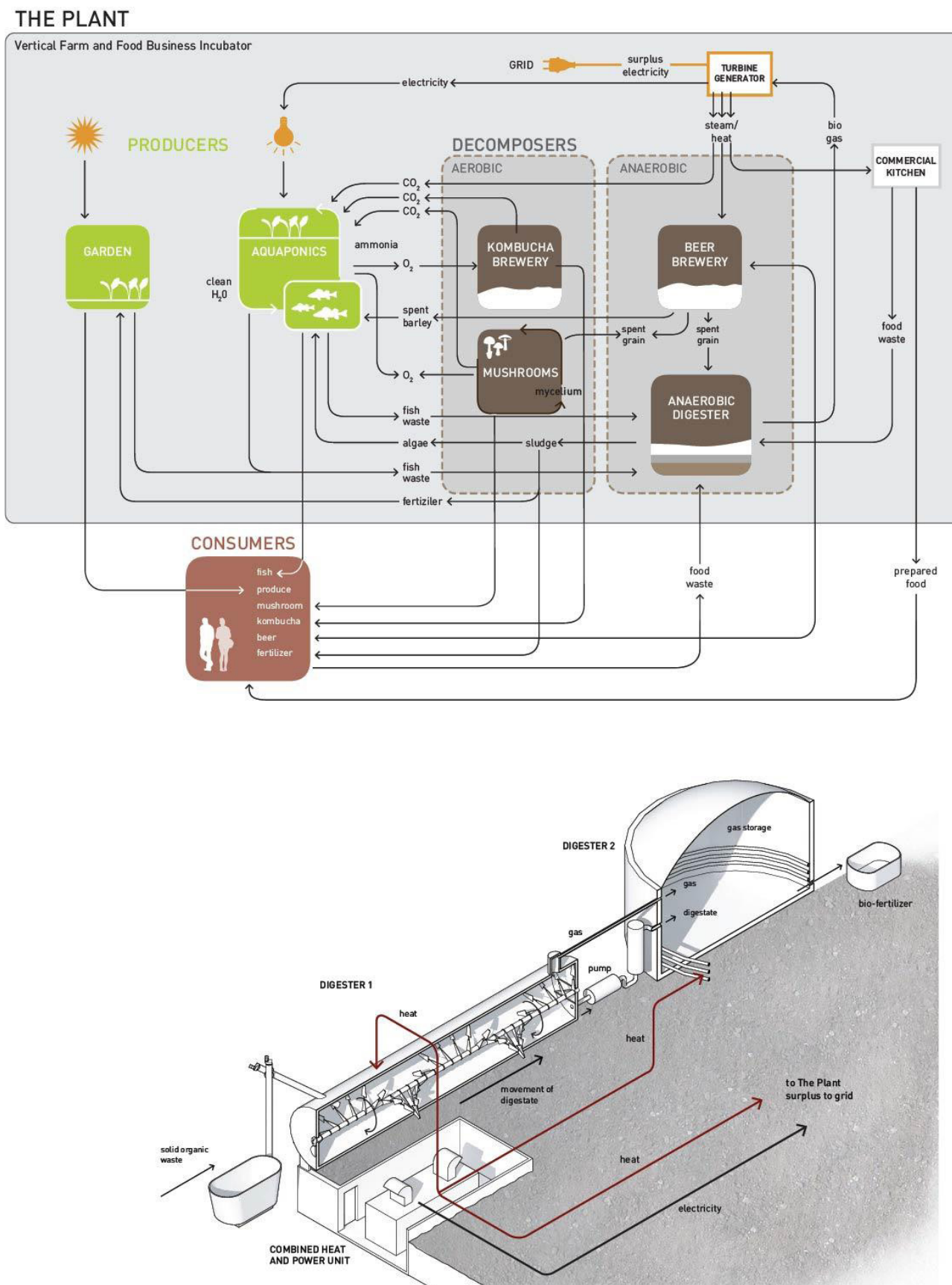
Figure 3: The Plant Chicago Anaerobic Digester and System Integration Diagram, Creating Urban Agricultural Systems (Proksch 2017)
