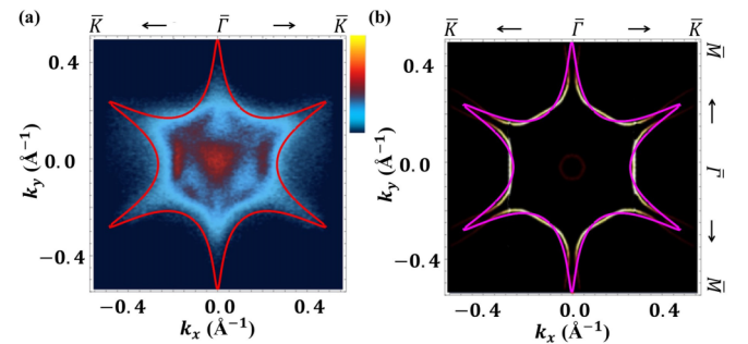
FIG. 4. Fit results with Eq. (1) to the TSS Fermi surface of \text{Bi}_4\text{Te}_3 with \text{Bi}_2\text{Te}_3 termination (a) to the experimental data with h\nu = 21.2 eV ( \lambda = 27.77 \text{ \AA}^2 and A = 2.668 \text{ \AA} ) and (b) to the DFT data (at the experimental E_F ; \lambda = 41.02 \text{ \AA}^2 and A = 2.110 \text{ \AA} ).
