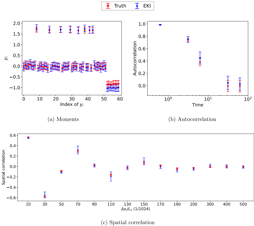
Fig. 26. Comparison between the data from the true system and results of the first sparse EKI, including (a) first four moments, (b) autocorrelation at x=0 , and (c) time-averaged spatial correlation.
