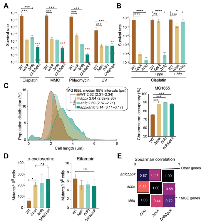
Fig. 2. Hfq and polyP display epistatic relationship in vivo. (A) Survival assay of MG1655 wt, \Delta ppk , \Delta hfq , and \Delta hfq\Delta ppk upon exposure cisplatin (4 \mu\text{g/ml} ), MMC (1 \mu\text{g/ml} ), phleomycin (0.25 \mu\text{g/ml} ), or UV (25 \text{J/m}^2 ). Error bars show 95% credible intervals. Comparisons are scored on the basis of the posterior probability of a difference in parameters in the observed direction: * P > 0.95 ; *** P > 0.999 . The red dashed lines indicate the predicted survival if the effects of the two single mutants were log additive. (B) Survival assay of WT, \Delta ppk , or \Delta hfq carrying either an empty plasmid (–) or a plasmid overexpressing ppk ( ppk^+ ) or hfq ( hfq^+ ) upon exposure to cisplatin (4 \mu\text{g/ml} ). Error bars denote 95% credible intervals, with * markings based on the posterior probability of a difference in parameters in the observed direction: * P < 0.95 ; **** P < 0.9999 . (C) Left: Cell size distribution of MG1655 wt ( n = 8670 ), \Delta ppk ( n = 8089 ), \Delta hfq ( n = 5875 ), or \Delta hfq\Delta ppk ( n = 5954 ). Right: Associated space occupied by the nucleoid in each mutant under nonstress condition; confidence intervals are obtained on the basis of bootstrapping of the observed cell-level data, and significance calling is performed between each genotype and WT using a Wilcoxon rank sum test (*** P < 0.005 ). (D) Mutant frequencies of WT, \Delta ppk , \Delta hfq , and \Delta hfq\Delta ppk strains upon growth on D-cycloserine or rifampin. (E) Gene expression analysis of MG1655 WT, \Delta ppk , \Delta hfq , and \Delta hfq\Delta ppk . Spearman correlation between phenotypes for “other genes” (continued box, upper triangle) or “MGE genes” (dashed box, lower triangle); all correlations are significant ( P < 10^{-5} in all cases). RNA-seq differential expression analysis on all genotypes is compared to WT for cells grown in glucose minimal medium (corresponding to the non-cisplatin-treated condition in Fig. 1A).
