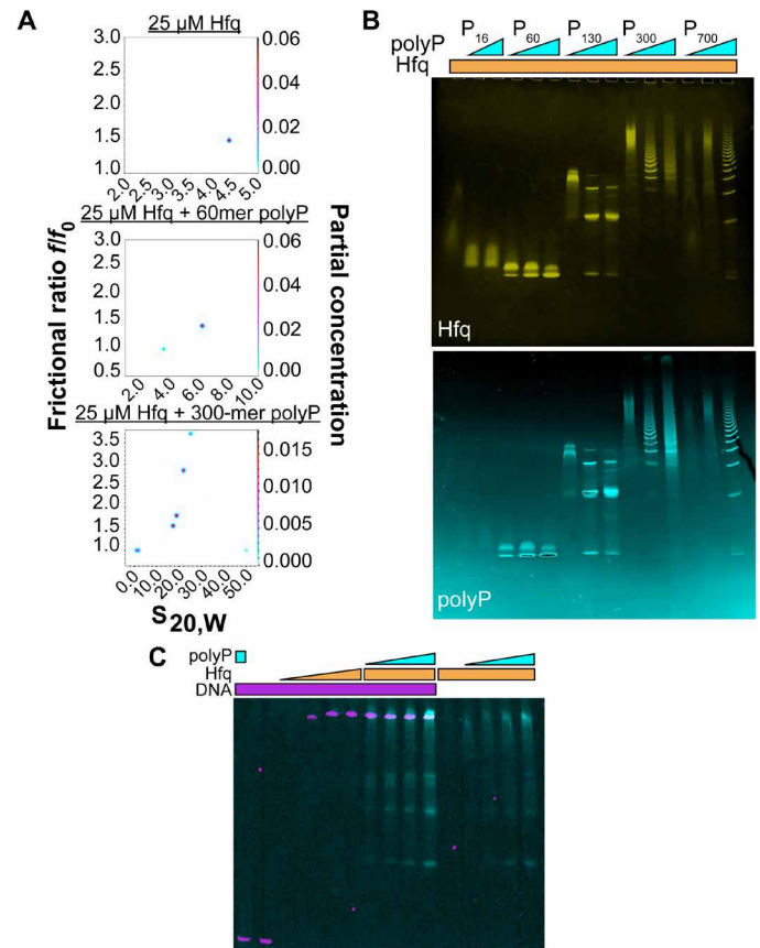
Fig. 4. In vitro interactions of Hfq, polyP, and DNA. (A) Two-dimensional analysis plots of frictional ratio f/f_0 versus sedimentation coefficient S for 25 \mu M Hfq \pm 250 \mu M polyP 60 or polyP 300 . The color in the z dimension represents the abundance of each species according to the partial concentration as indicated in the right y axis. (B) Mobility of Hfq (25 \mu M) on native gels without (lane 1) or with 65, 125, or 250 \mu M of various polyP chain lengths. PolyP 16 was used at 125 and 250 \mu M only (lanes 2 and 3). Gels were stained with 4',6-diamidino-2-phenylindole (DAPI) to visualize polyP (cyan) followed by Coomassie staining to visualize Hfq (yellow). (C) Overlay of EMSA using FAM-labeled ybcK -DNA (75 nM) in the presence of 30 \mu M Alexa Fluor 647 (AF647)-polyP 300 (lane 1); in the absence of additives (lane 2); or in the presence of 5, 10, 17.5, or 25 \mu M Hfq (lanes 3 to 6). AF647-polyP 300 (in P_i units) was added at 10, 15, 20, or 30 \mu M to 25 \mu M Hfq and DNA (lanes 7 to 10) or 25 \mu M Hfq only (11–15). Gels were stained with Coomassie to detect Hfq (fig. S4B).
