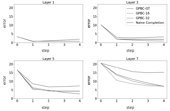
Fig. 9: Quantitative Analysis. We show quantitative results on our synthetic dataset for our GPBC approach at two different threshold values (16 and 32), GPBC with random groundtruth corners gradually uncovered, and naive image completion. The x -axis corresponds to the number of steps for the iteration completion and the y -axis shows the error (Eq. 5) between the ground truth completion and the predicted completion. Compared to the baseline shown in red, our proposed model reduces the error faster (after step 1) and yields a final prediction with a smaller error.
