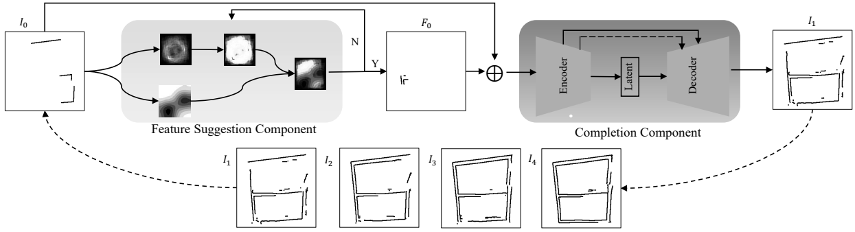
Fig. 2: Pipeline. Iterates over a Feature Suggestion Component and a Completion Component.
