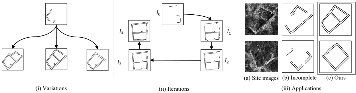
Fig. 1: Building Contour Completion. (i) Our approach supports pluralistic completions. (ii) User is able to complete highly incomplete building contours in just a few iterations. (iii) We demonstrate on real-world archaeological sites.
