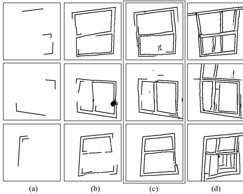
Fig. 20: Different Completion Levels. We show (a) incomplete footprints, (b-d) completion results generated by the completion model trained under 25%, 50% and 100% completion levels, respectively.
