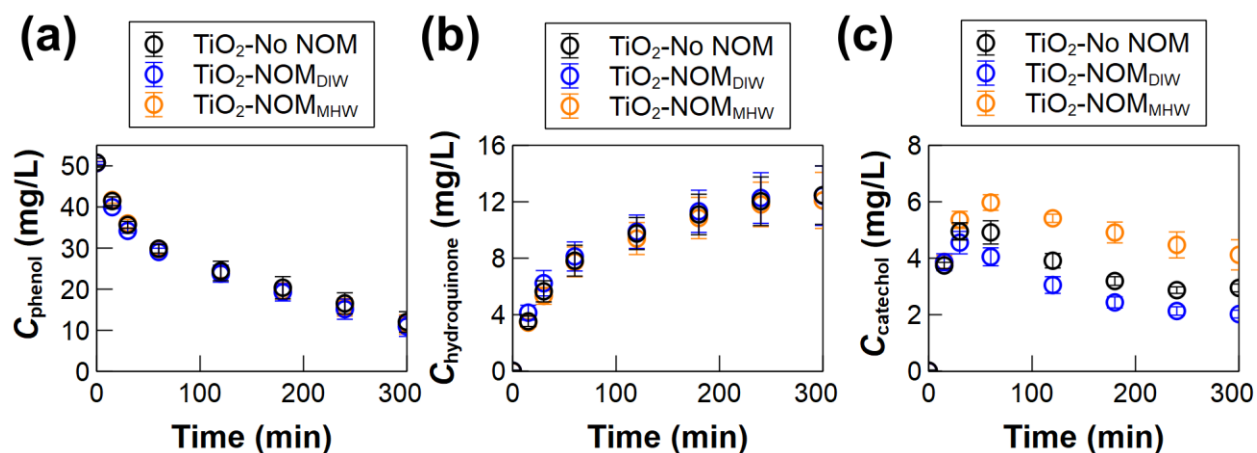
Figure 3. Degradation of 50 mg/L phenol (a), and formation and/ or degradation of hydroquinone (b) and catechol (c) using 100 mg/L of TiO 2 -No NOM, TiO 2 -NOM DIW , or TiO 2 -NOM MHW (all in 10 mM phosphate buffer). No phenol losses were observed in dark controls after 300 min (not shown). Error bars represent standard deviation across triplicate experiments.
