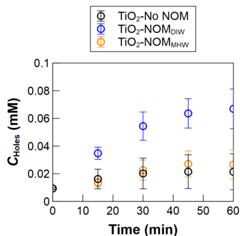
Figure 6. Quantification of holes generated upon irradiation of the \text{TiO}_2 NPs in 10 mM phosphate. Error bars represent standard deviation across four replicate experiments.
