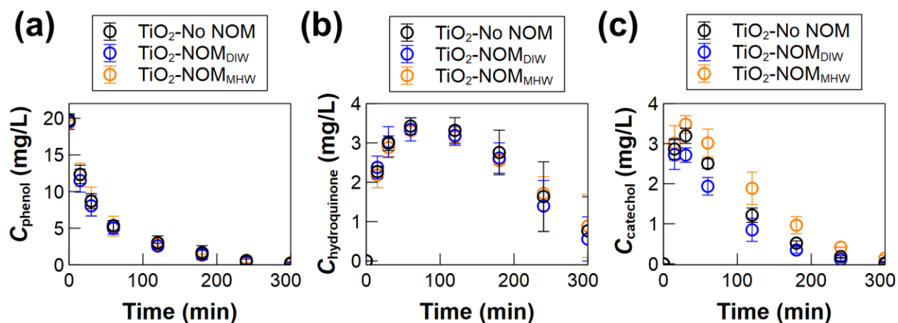
Figure 2. Degradation of 20 mg/L phenol (a), and formation and/ or degradation of hydroquinone (b) and catechol (c) using 100 mg/L of TiO 2 -No NOM, TiO 2 -NOM DIW , or TiO 2 -NOM MHW (all in 10 mM phosphate buffer). No phenol losses were observed in dark controls after 300 min (not shown). Error bars represent standard deviation across triplicate experiments.
