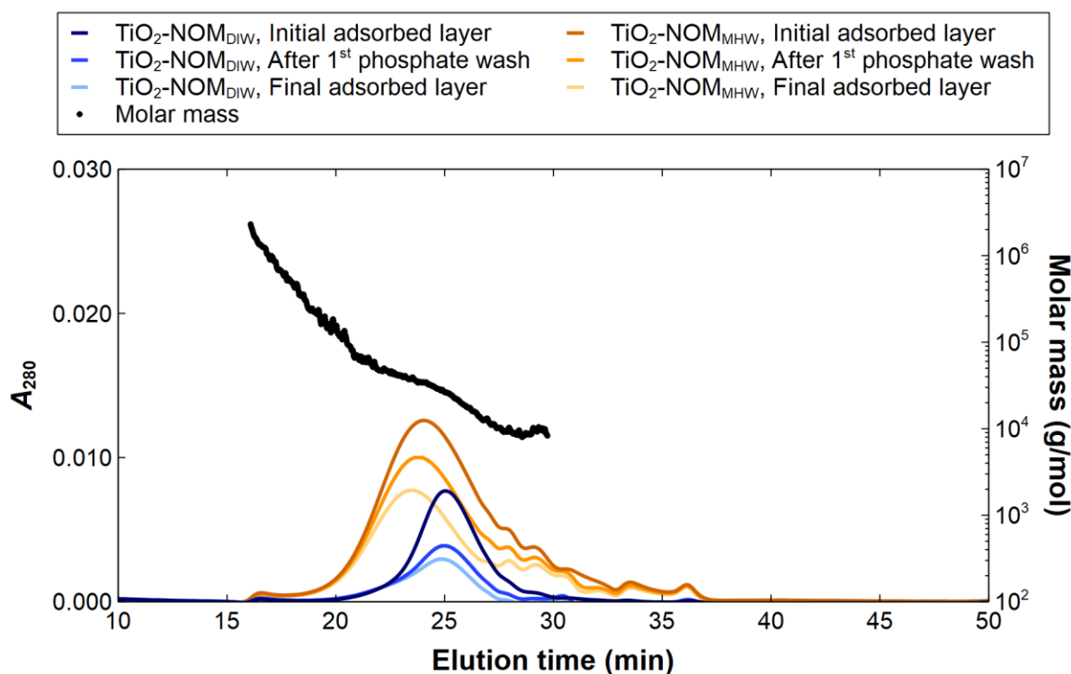
Figure 1. NOM species adsorbed to the \text{TiO}_2 NPs from DIW or MHW, before and after phosphate washes, as identified by difference chromatogram analysis of SEC-UV data. The estimated molar mass of NOM across the elution time was determined by SEC with multi-angle light scattering (MALS) on a 3 g/L NOM sample (method details in the SI).
