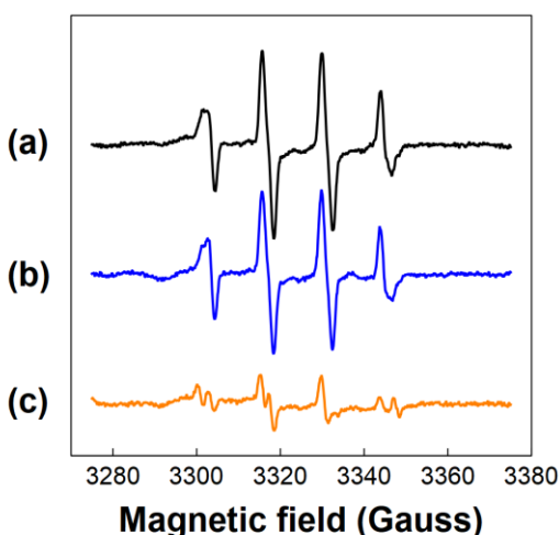
Figure 5. EPR spectra of BMPO-radical adduct(s) formed in the UV irradiation reactions with \text{TiO}_2\text{-No NOM} (a); \text{TiO}_2\text{-NOM}_{\text{DIW}} (b); and \text{TiO}_2\text{-NOM}_{\text{MHW}} (c).
