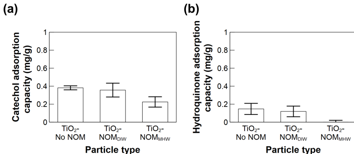
Figure 4. Adsorbed mass of catechol (a) and hydroquinone (b) onto \text{TiO}_2 -No NOM, \text{TiO}_2 - \text{NOM}_{\text{DIW}} , and \text{TiO}_2 - \text{NOM}_{\text{MHW}} from 5 mg/L initial concentrations of the catechol and hydroquinone in 10 mM phosphate buffer. Error bars represent standard deviation across triplicate experiments.
