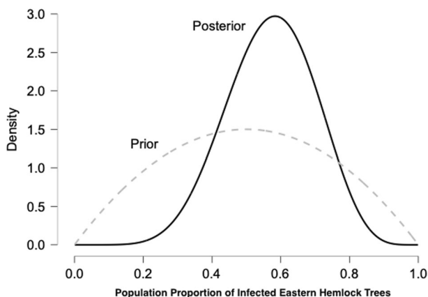
Fig. 1 Example of using Bayes' theorem to update prior information in light of new evidence.
