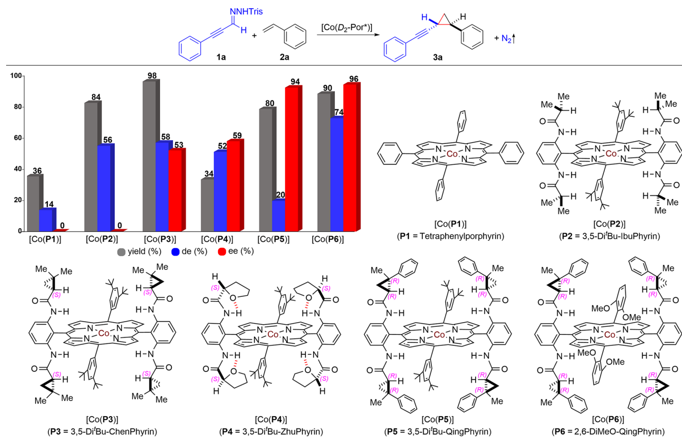
Scheme 2. Ligand Effect on Co(II)-Based Catalytic System for Olefin Cyclopropanation with Alkynyldiazomethane a
