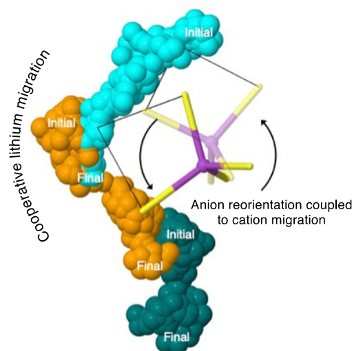
Figure 2: Relationship between cage dynamics and ion transport in a glassy \text{Li}_3\text{PS}_4 . Li-ion migration event involving the displacement of three Li-ions and a neighboring \text{PS}_4 anion. The position of the anion is shown before and after migration using transparent and opaque shading. Adapted with permission from reference 21. Copyright 2021 Cell Press.
