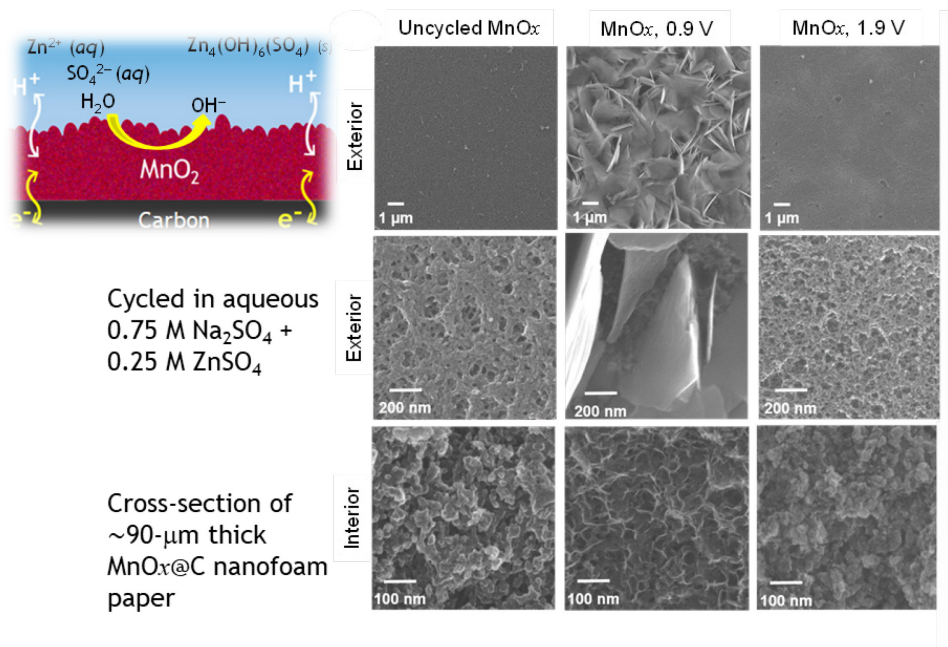
Figure 3: Schematic depicting \text{H}^+ insertion into \text{MnO}_x from mild aqueous electrolyte containing \text{Zn}^{2+} ; ex situ scanning electron microscopy survey of an architected cathode prepared by “painting” the walls of carbon nanofoam with nanometric \text{MnO}_x to create a cathode that distributes the pH-driven precipitation of salt (zinc hydroxy sulfate) not just at the exterior but throughout the interior of the macroscale thick carbon nanofoam upon changes in interfacial pH upon proton insertion (at 0.9 V vs. Zn) and deinsertion at 1.9 V. Adapted with permission from reference 26. Copyright 2018 Springer-Nature.
