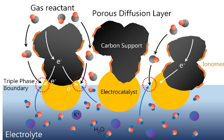
Figure 1: Schematic depicting the complexity of a typical electrode-electrolyte interface in a gas-fed flow reactor. Electrocatalyst particles are mixed with ionomers (for charge conductivity), and then sprayed onto a porous gas diffusion layer (for gas diffusion and electron conductivity) to form a typical gas diffusion electrode.
