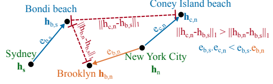
Figure 3: Illustration of the usefulness of our analogy-inspired encoding. The two beaches have similar relationships to their city, hence they should be more similar than other neighborhoods—even though their absolute similarity may be low.
