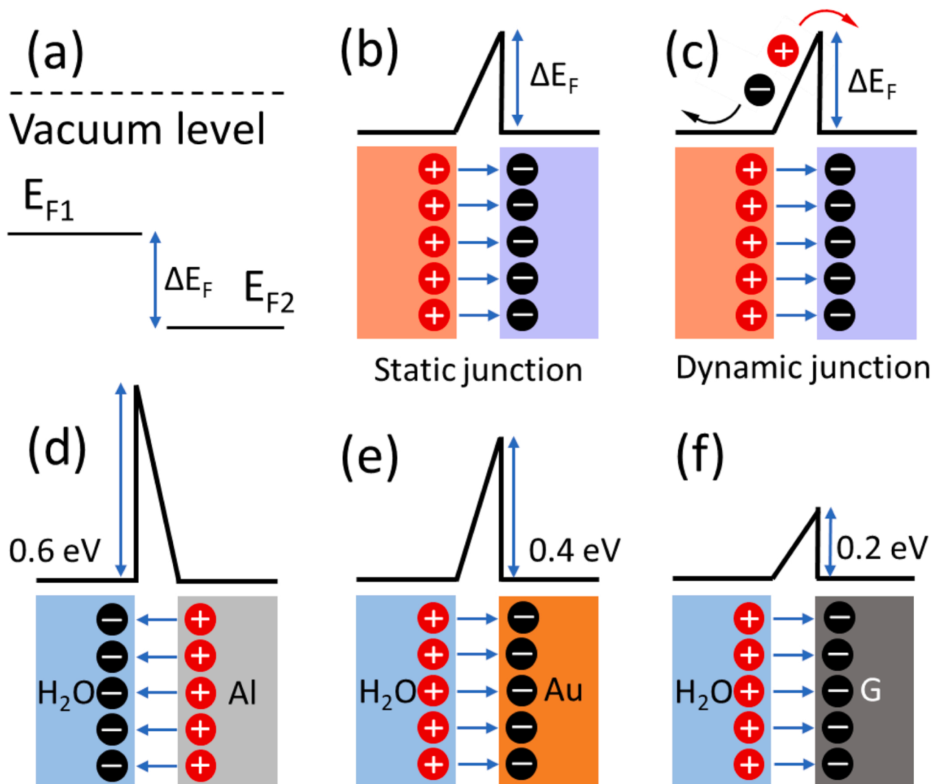
Fig. 4. Generalized dynamic junction theory for DC generation. (a) Two materials with different Fermi levels. (b) Space charge, built-in electric field and potential after two materials are in contact. (c) Separation of electron and hole in a dynamic junction to generate a DC. (d-f) Schematics of space charge and built-in potentials at the interfaces of (d) water-Al, (e) water-Au, (f) water-graphene based on their Fermi levels in Fig. 3a. G indicates graphene.
