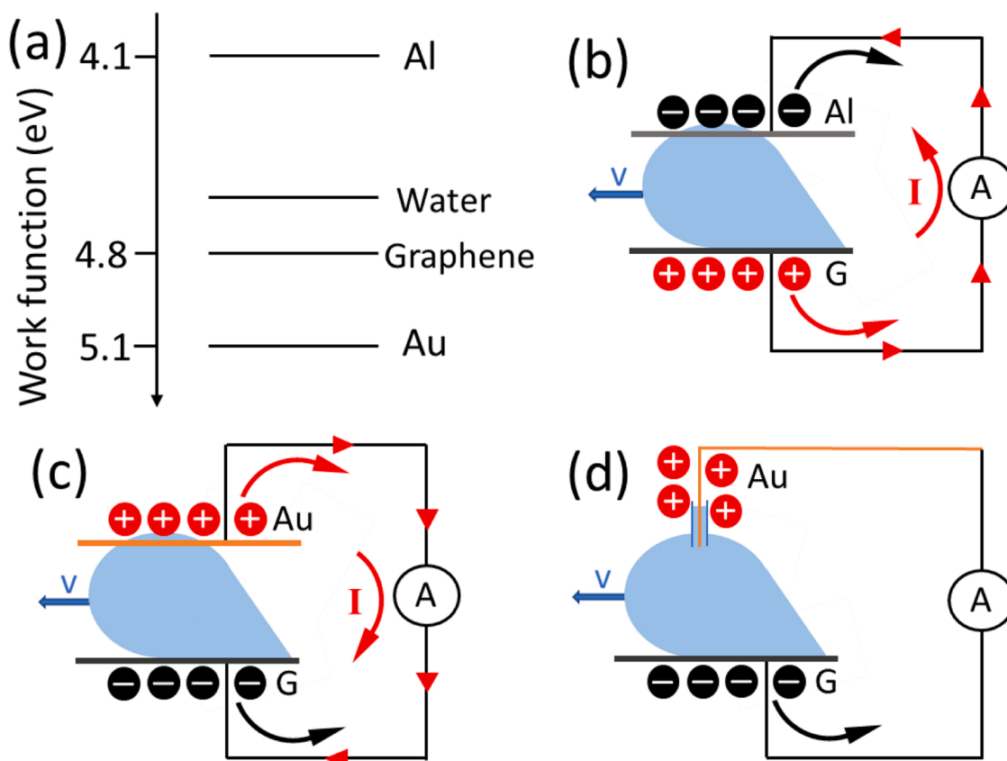
Fig. 3. Failure of charge-discharge theory. (a) Fermi levels of graphene, water, Al, and Au. (b-c) Successful charge-discharge description of DC between graphene and suspended (b) Al wires and (c) Au wires. (d) Expected DC from the charge-discharge theory when applied to the moving Au wire.
