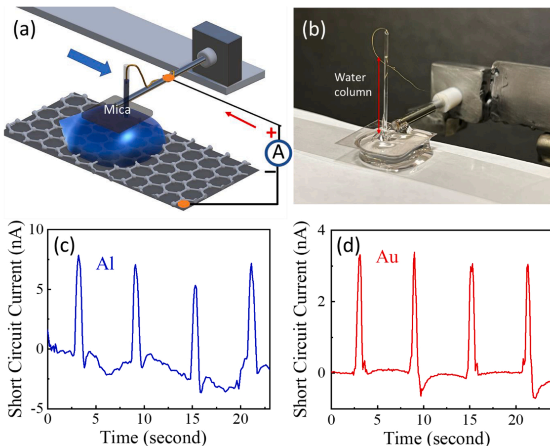
Fig. 2. DC between graphene and a metal wire moving with a droplet. (a) Schematic of the experimental setup. (b) Picture of the setup with an Au wire in a capillary tube. (c-d) The current between graphene and (c) Al wire and (d) Au wire when the water droplet moves back and forth.
