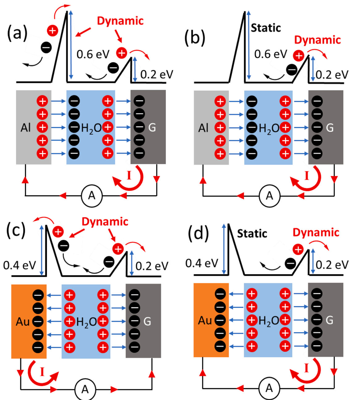
Fig. 5. Application of generalized dynamic junction theory to DC generators in Figs. 1 and 2. (a-b) Current generations in graphene-Al generators with (a) suspended and (b) moving Al wires. (c-d) Current generations in graphene-Au generators with (c) suspended and (d) moving Au wires.
