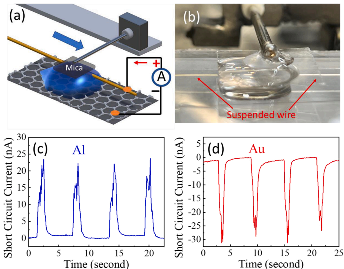
Fig. 1. DC between graphene and a suspended metal wire with a moving water droplet (a) Schematic of the experimental setup. (b) Picture of the setup. (c-d) The current between graphene and (c) Al wire and (d) Au wire when the water droplet moves back and forth. A positive current indicates current from graphene to wire through the current meter.
