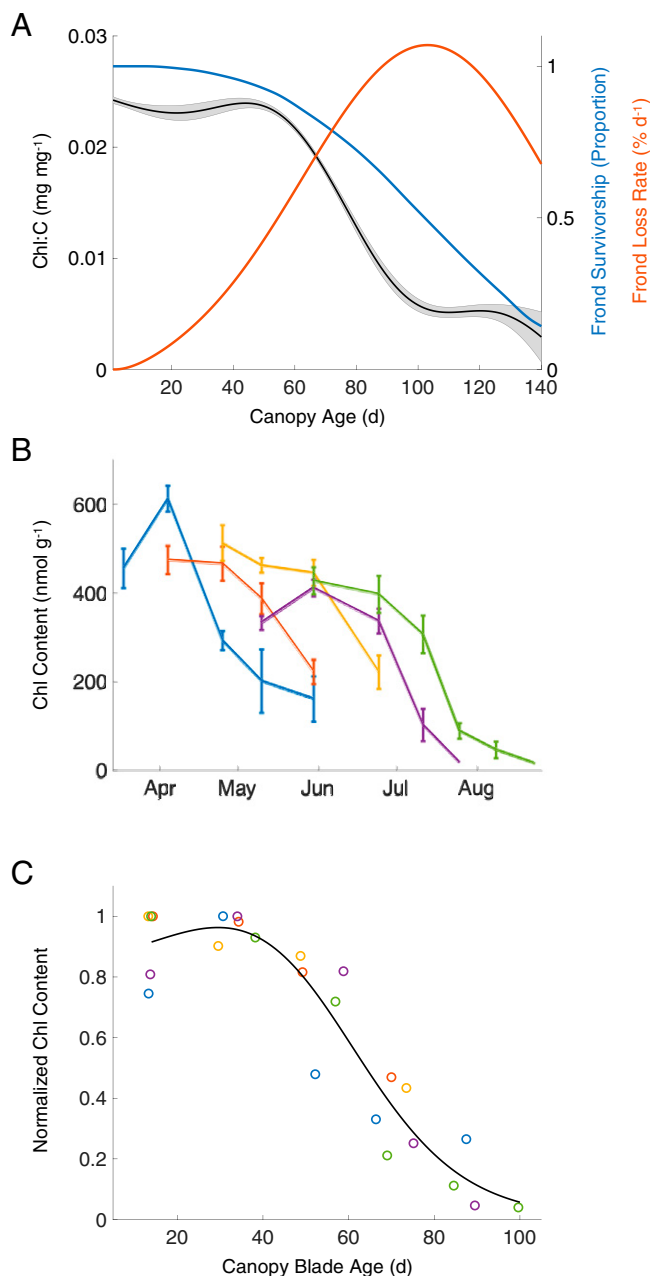
Fig. 3. (A) The nonlinear relationship between canopy age and Chl:C across all three image dates in 2015 for the large kelp forest in Fig. 2 (black curve; the gray shaded area represents 2× SE). The proportional frond survivorship (blue curve) and the loss rate of fronds (red curve) across three kelp forests in the SBC; synthesis of data from ref. 9. (B) Canopy chlorophyll a content as a function of age across five frond cohorts sampled in the SBC in 2019. Errors bars show SE. (C) The relationship between chlorophyll a content, normalized to the maximum of each frond cohort, and age for the five frond cohorts shown in B. Points are slightly jittered for visibility and colored to correspond to their respective frond cohort.
