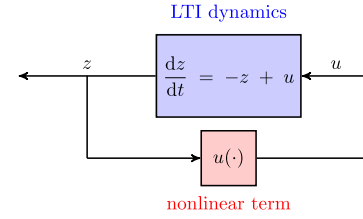
Fig. 1. Both the proximal gradient flow dynamics (15) and the DR splitting dynamics (26) can be represented via feedback interconnections of stable LTI systems with nonlinear terms that possess certain structural properties.
