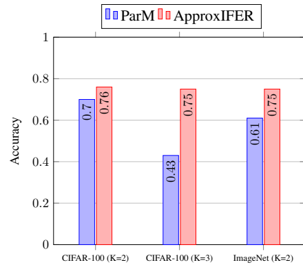
Figure 9: Comparison of the accuracy of ApproxIFER with the degraded mode accuracy of ParM for CIFAR-100 for K = 2, 3 , S = 1 and E = 0 , and ImageNet datasets for K = 2 , S = 1 and E = 0 . The network architectures considered are ResNet-50 and ResNet-152 for CIFAR-100 and ImageNet, respectively.
