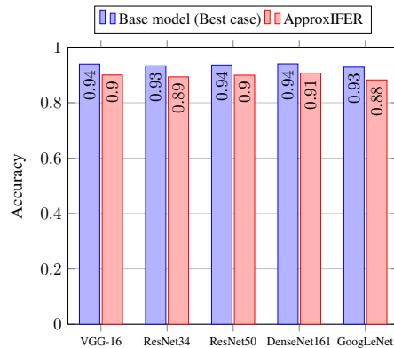
Figure 11: Accuracy of ApproxIFER on CIFAR-10 and various network architectures for K = 12 , S = 0 and E = 2 .
