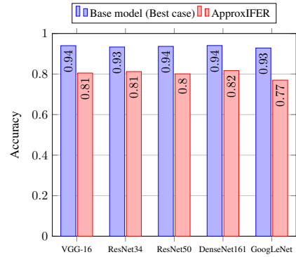
Figure 8: Accuracy of ApproxIFER on CIFAR-10 and with various network architectures for K = 8 , S = 1 .
