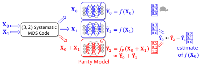
Figure 1: An example of ParM is illustrated with K = 2 queries denoted by \mathbf{X}_0 and \mathbf{X}_1 . The goal is to compute the predictions \mathbf{Y}_0 = f(\mathbf{X}_0) and \mathbf{Y}_1 = f(\mathbf{X}_1) . In this example, the system is designed to tolerate one straggler. Worker 1 and worker 2 have the model deployed by the prediction serving system denoted by f . Worker 3 has the parity model f_P which is trained with the ideal goal that f_P(\mathbf{X}_0 + \mathbf{X}_1) = f(\mathbf{X}_0) + f(\mathbf{X}_1) . In this scenario, the first worker is slow and f(\mathbf{X}_0) is estimated from f(\mathbf{X}_1) and f_P(\mathbf{X}_0 + \mathbf{X}_1) .
