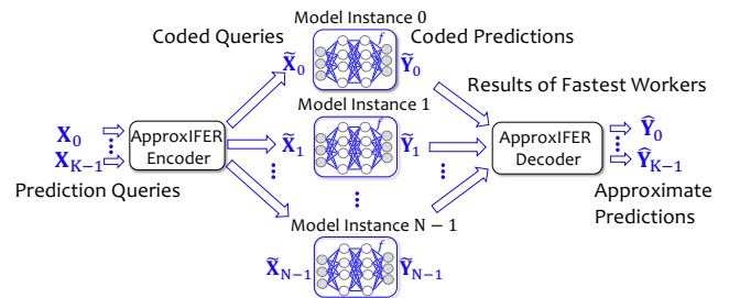
Figure 4: In ApproxIFER, all workers have the model deployed by the system f , no parity models are required and only an encoder and a decoder are added on top of the conventional replication-based prediction serving systems. The K input queries \mathbf{X}_0, \dots, \mathbf{X}_{K-1} are first encoded. The predictions are then performed on the coded queries. Finally, the approximate predictions \tilde{\mathbf{Y}}_0, \dots, \tilde{\mathbf{Y}}_{K-1} are recovered from the fastest workers.
