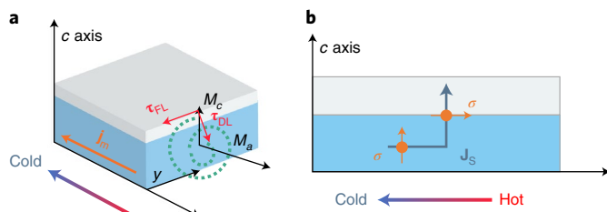
Fig. 4 | Schematic of the spin swapping mechanism at the interface of a c-axis oriented LaFeO 3 crystal and a heavy metal. a , Schematic of the spin-torque swapping effect in c-axis oriented LaFeO 3 /Pt with an in-plane temperature gradient along the x direction. The magnon current \mathbf{j}_m is along the temperature gradient (the magnonic spin current is in the opposite direction to the magnon because it carries spin -1 ). The dotted line shows the trajectory of the magnetic moment. \tau_{DL} ( \tau_{FL} ) is the damping-like (field-like) spin torque induced by the interfacial DMI which contributes to swapping the net magnetic moment M_c of \Gamma_4 to an in-plane moment M_a of \Gamma_2 . The x component of M_a accompanied by a z component of spin-torque-induced spin current then contributes to a detectable voltage along the y direction by the ISHE. b , Schematic of a 90° rotation of the spin index and the transformation of an in-plane magnon current to an out-of-plane spin current.
