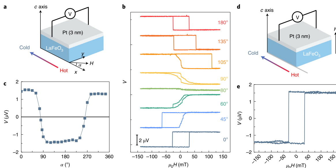
Fig. 3 | Magneto-thermoelectric measurements on the c-axis oriented LaFeO 3 /Pt with an in-plane temperature gradient. a , Schematic of the transverse thermal voltage measurement in c-axis oriented LaFeO 3 /Pt with an in-plane temperature gradient along the x direction and an in-plane magnetic field. b , Magnetic field dependence of the transverse thermovoltage in c-axis oriented LaFeO 3 /Pt for various in-plane field angles (see Supplementary Fig. 7a,b for the results from 180° to 360°). c , Transverse thermovoltage at magnetic saturation as a function of in-plane field angle. d , Schematic of transverse thermovoltage measurement in c-oriented LaFeO 3 /Pt with in-plane temperature gradient and magnetic field along z direction. e , Magnetic field dependence of the transverse thermovoltage from the device in d . Such strong and clear signals have not been previously reported in any system with an in-plane temperature gradient.
