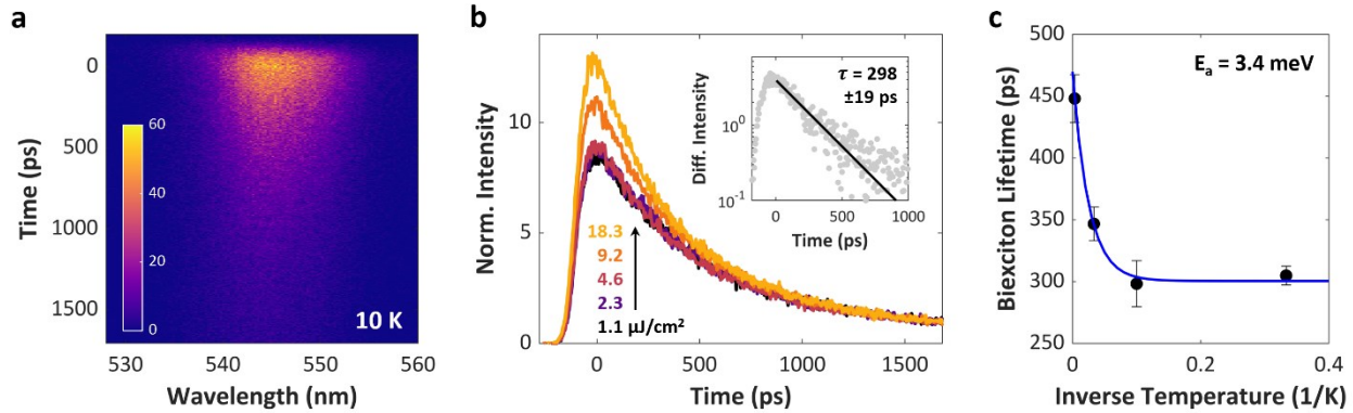
Figure 2. Fluence-dependent time-resolved PL of 5.5 ML thick CdSe NPLs dispersed in a 1:1 mixture of hexanes to methylcyclohexane. (a) Representative trPL data at 10 K. The color scale indicates number of detected photons per pixel. (b) Example trPL data at 10 K for a range of indicated fluences, integrated across the wavelength region of interest shown in (a) and normalized at late time (near 1500 ps). The biexciton lifetime was determined by subtracting such normalized single exciton dynamics from the higher power data. The result of the subtraction procedure, shown in the inset, yields monoexponential data that can be fitted to determine the biexciton lifetime. (c) Biexciton lifetime
