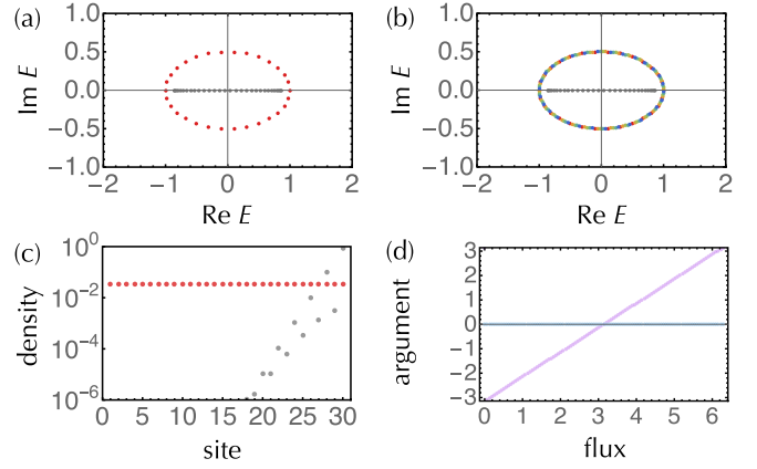
FIG. 1. Interacting Hatano-Nelson model with one particle ( L = 30 , N = 1 , \gamma = 0.5 ). (a) Complex spectra under the periodic boundary conditions (red dots) and open boundary conditions (black dots). (b) Complex spectra under the periodic and open boundary conditions in the presence of the flux \phi \in \{0, 2\pi/5, 4\pi/5, 6\pi/5, 8\pi/5\} . (c) Spatial distributions of particle numbers for an eigenstate with E = -0.10 - 0.50i under the periodic boundary conditions (red dots) and an eigenstate with E = -0.04 under the open boundary conditions (black dots). (d) Arguments of the determinants of \hat{H}_1(\phi) - E as a function of the flux \phi for E = 0 (purple dots, W = 1 ) and E = -1.5 (blue dots, W = 0 )
