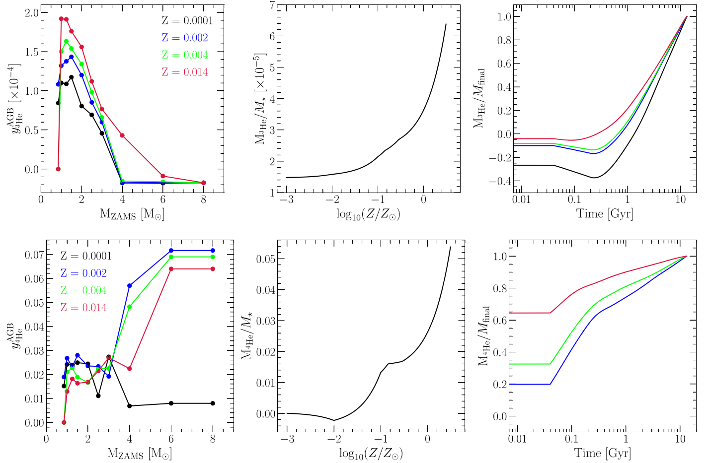
Figure 6. The {}^3\text{He} and {}^4\text{He} yields of asymptotic giant branch (AGB) stars (top and bottom panels, respectively). Left: fractional yield as a function of the zero-age main-sequence (ZAMS) stellar mass. The yield of {}^3\text{He} is dominated by the lowest-mass stars, while the yield of {}^4\text{He} is dominated by intermediate- and high-mass stars. Middle: IMF-integrated yield as a function of metallicity for a simple stellar population, normalized by the total stellar mass. The yields of both {}^3\text{He} and {}^4\text{He} are greater for higher-metallicity stellar populations. Right: fractional time evolution of {}^3\text{He} and {}^4\text{He} for a simple stellar population. The {}^3\text{He} yield is dominated by the lowest-mass stars. As a result, radial migration is expected to be important for understanding the galactic chemical evolution of {}^3\text{He}/{}^4\text{He} . We note that the Z = 0.0001 curve is not shown in the bottom-right panel for {}^4\text{He} , because extremely metal-poor massive stars net destroy more {}^4\text{He} than AGB stars net produce.
