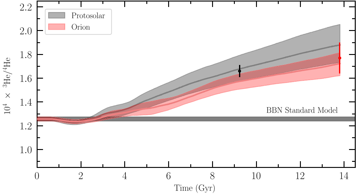
Figure 9. Same as Figure 8, but the VICE model shown here assumes the Standard Model ^3\text{He}/^4\text{He} ratio and allows the strength of the outflow prescription to vary as a free parameter. The best-fit models scale the default outflow mass-loading efficiencies upward by a factor f_s = 1.7 .
