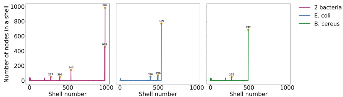
Fig. 4. Validation of KOMB on simulated data with a real genomic backbone. Combined KOMB profile of E. coli (intra: 400 \times 400 bp, inter 500 \times 500 bp) and B. cereus (intra: 200 \times 400 bp, inter 500 \times 500 bp) repeats (Left), E. coli single genome (Middle), and B. cereus single genome (Right). For the combined profile of both bacteria (L), there is a clear formation of peaks close to position 1000 (984 and 979), which indicate the inter-genomic repeats, and peaks at shell numbers 277, 396 and 540. We also plot the individual profiles of E. coli and B. cereus . For E. coli (M) we see three peaks at 396, 496 and, 539 given its higher copy number of intra-genomic repeats (400). For B. cereus , we observe peaks at 276 and 492 signalling its intra- and inter-genomic repeats, respectively.
