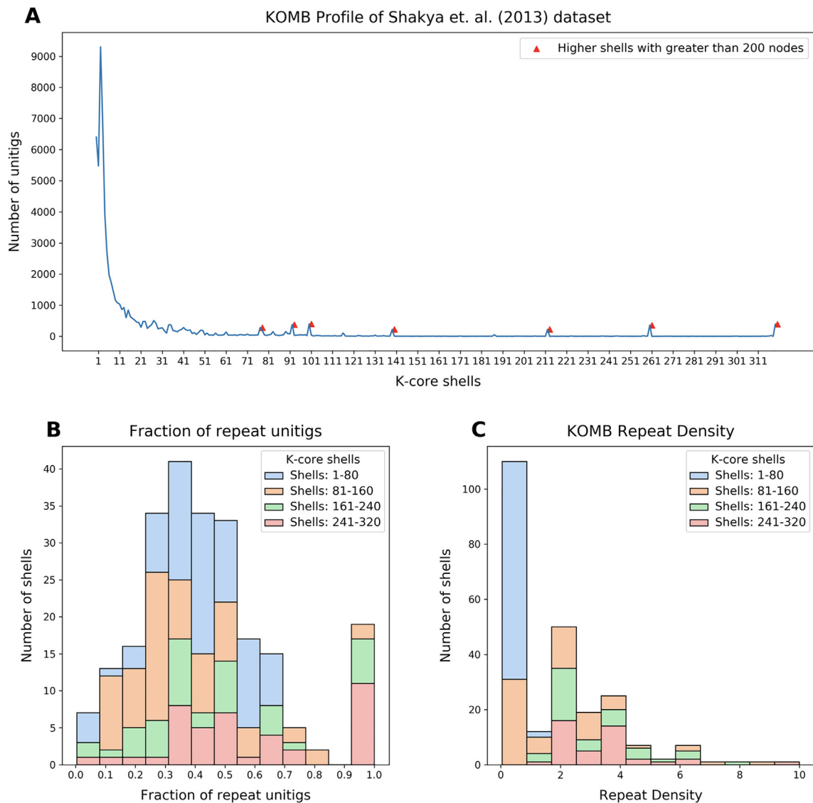
Fig. 6. Characterization of a synthetic metagenome sample using KOMB. A. KOMB profile of the Shakyra et al. (2013) dataset representing the shell number on the x-axis and the number of units in the y-axis. Red triangles indicate higher shells with greater than 200 nodes, which represent clique or clique-like regions in the hybrid unitig graph. B. Histogram representing the fraction of units in each of the shells that are repeats as determined by comparing with the nucmer output. C. KOMB repeat density is defined as the average copy number per number of genomes for the repeat units in the shell (see Eq. 2). Larger shells have repeats with high copy number and more specific to a single (or group of related) organisms. For figures B. and C., shell 0 (disconnected nodes) and shells that contained no unitigs are not considered. Shells are split into four different groups (1–80, 81–160, 160–240, 241–320) for visualization.
