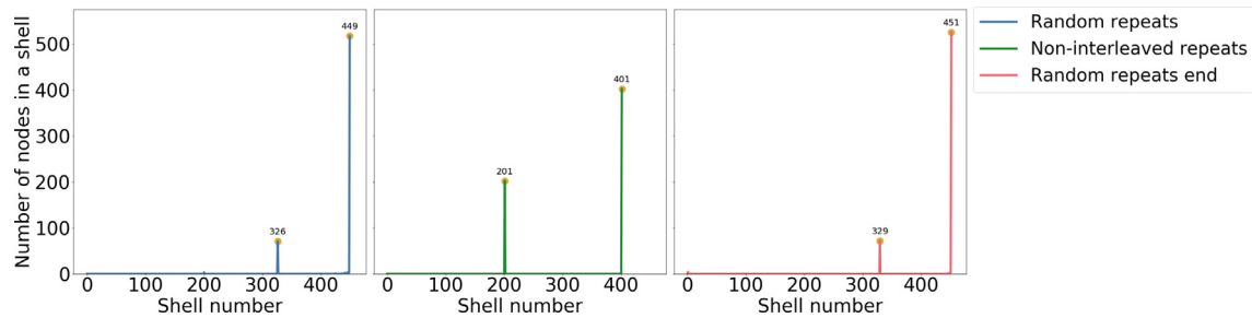
Fig. 3. Validation of KOMB on simulated data. KOMB profiles on a random backbone with 200 \times 400 bp and 400 \times 200 bp identical repeats when randomly inserted (L), inserted at different ends (M), and inserted in the same end (R). The x-axis represents the shell number and the y-axis represents number of nodes (units). In the ideal case (M) where the units have the same repeats at its end we observe peaks at 201 and 401 respectively. Interleaving repeats randomly (L) causes a shift in the peaks towards higher shells to 326 and 449, respectively. Further, inserting both kinds of repeats at the same end (R) results in a similar shift with peaks occurring at 329 and 451.
